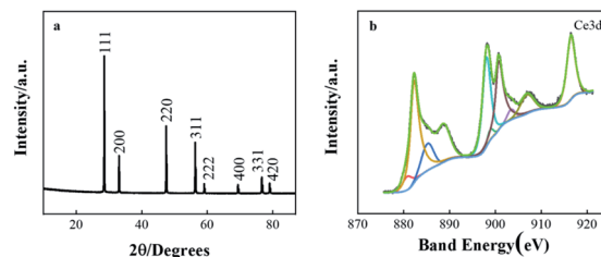
Fig. 4 (a) XRD patterns for cerium oxide deposited film on FTO surface; (b) X-ray photoelectron spectra of \text{Ce}_3\text{d} .
