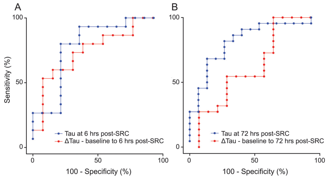
(A) Blue curve represents the receiver operating characteristic (ROC) of plasma tau measured 6 hours after SRC for predicting RTP. The area under the curve (AUC) was 0.81; 95% confidence interval (CI) 0.62-0.97, p = 0.01 . The red curve represents the ROC of the participant-specific change in plasma tau from baseline to 6 hours after SRC for predicting RTP. AUC was 0.80; 95% CI 0.57-0.94, p = 0.02 . (B) Blue curve represents the ROC of plasma tau measured 72 hours after SRC for predicting RTP. The AUC was 0.82; 95% CI 0.68-0.96, p < 0.01 . The red curve represents the ROC of the participant-specific change in plasma tau from baseline to 72 hours after SRC for predicting RTP. AUC was 0.74; 95% CI 0.58-0.90, p = 0.20 .
