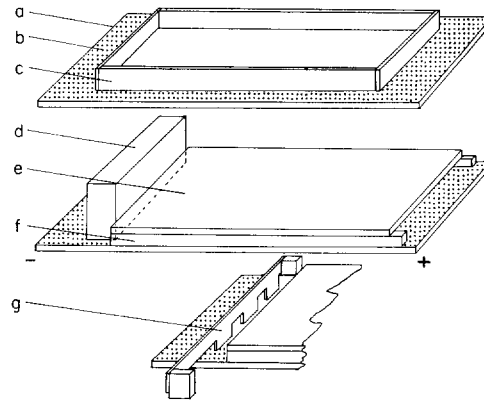
FIGURE 2 Design of discontinuous acrylamide gel plate: (a) ring, 1 cm wide, of 5% acrylamide gel; (b) ground glass projection slide 3\frac{1}{4} \times 4 inches; (c) plastic form, removable; (d) plastic divider; (e) glass cover plate, covering 7.5% running gel; (f) plastic spacers \frac{1}{8} inch thick; (g) mold for sample slots set in 5% spacer gel.
