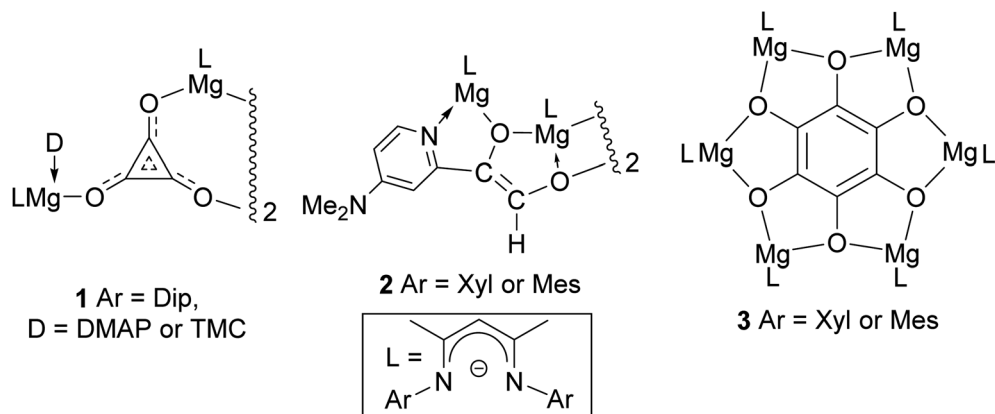
Fig. 1 Previously described products derived from the reductive homology of CO by neutral dimagnesium(I) compounds.
