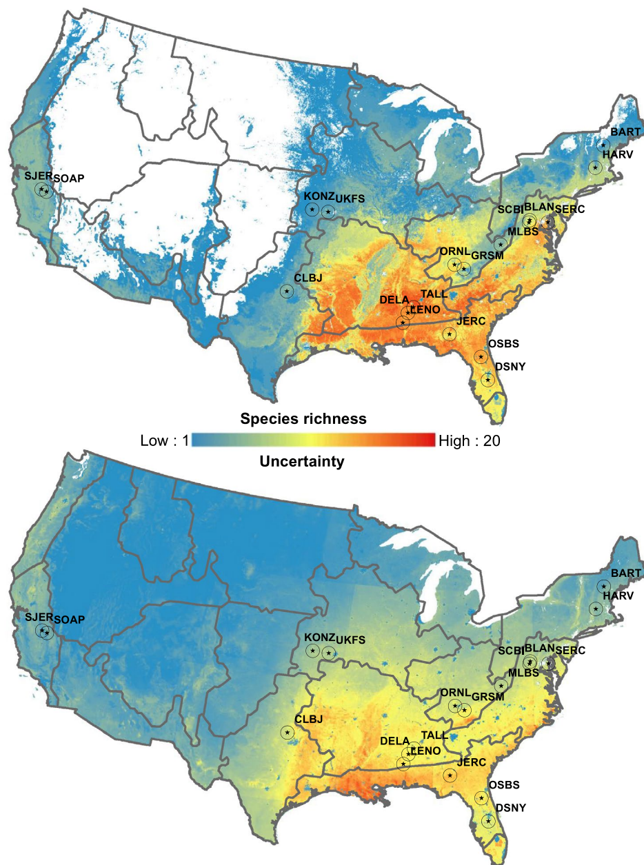
Figure 2. Macroecological patterns of the number co-occurring oak species (top panel) and uncertainty (low panel) estimated by stacking individual species distribution model binary predictions (S-SDMs). Numbers on the legend represent the number of co-occurring within each pixel. In addition, blue and red colors mean low and high species co-occurrence (uncertainty), respectively. Star symbols (and acronyms) on the map represent the nineteen NSF-NEON sites that have data of oak species assemblages. Overlaid gray polygons represent the NSF-NEON ecoclimatic domains. Map projection: Lambert Azimuthal Equal Area. Maps were generated using ArcGIS Desktop 10.6 ( https://desktop.arcgis.com/ ).
