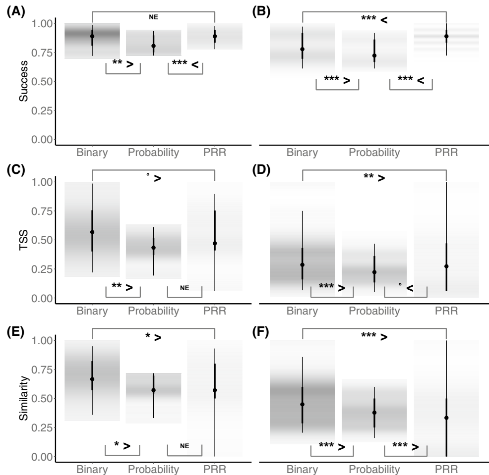
Figure 5. Accuracy of assemblage composition predictions at site and plot scales. Left panels (A,C,E) metrics at site scales and right panels (B,D,E) metrics at plot scale. Significant differences between stacking procedures (bS-SDM versus pS-SDM versus cS-SDM) were evaluated using Bayesian ANOVAs with NEON plot IDs as random effect (significance levels for the Maximum A Posteriori p-values are: *** p = 0 , ** p < 0.01 , * p < 0.05 , \bullet p < 0.1 , NE no evidence).
