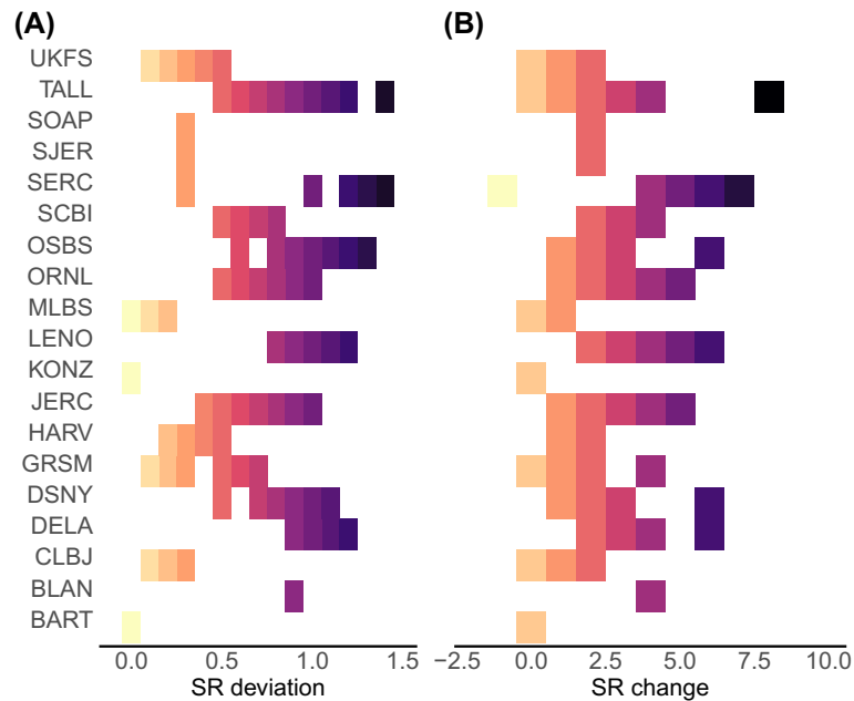
Figure 4. Accuracy of the number of co-occurring oak species predictions at site and plot scale. (A) Species richness deviation, measured as the absolute deviation in assemblage richness predictions divided by the maximum observed NEON plot species richness, where low and high values represent high and low accuracy respectively. (B) Species richness change, that represent the species loss or gain at plot scale. Negative values represent the number of species lost (underprediction) while positive values the gain of species (overprediction).
