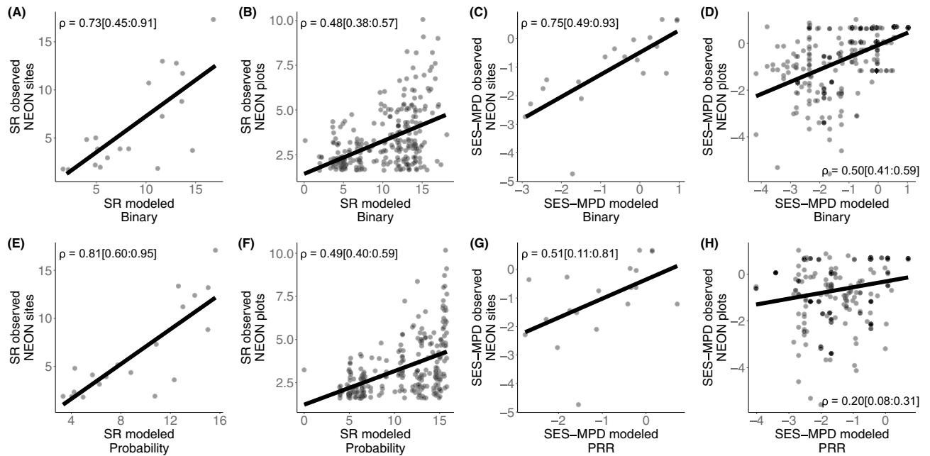
Figure 3. Predicted versus observed number of co-occurring oak species (left panels) and phylogenetic assemblage structure (right panels) at site and plot scales. Rho ( \rho ) values within each panel represent the median Pearson’s correlation coefficients estimated from posterior distribution and the 95% of credible intervals within brackets.
