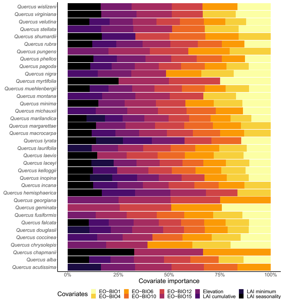
Figure 1. Covariate importance or the relative contributions (%) of the 10 covariates used for modeling the potential distribution of oak species in the Continental United States.
