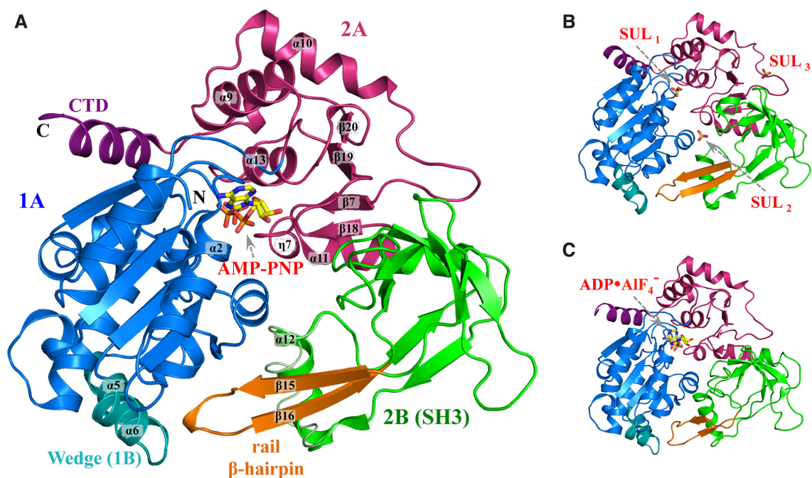
Figure 1. Structural overview of hPIF1. Cartoon representation of the hPIF1 helicase core domain. (A) The 1.13 Å hPIF1-AMP-PNP structure. Domains are coloured as 1A (blue), 2A (red) and 2B (green). Note the C-terminal domain (CTD, purple) and the functional wedge domain (1B, cyan) are structurally part of domain 1A. The rail \beta -hairpin (orange) is part of domain 2B (a SH3 domain). Secondary structure elements \alpha 2 , \alpha 5 , \alpha 6 , \alpha 9 , \alpha 10 , \alpha 11 , \alpha 12 , \alpha 13 , \beta 7 , \beta 15 , \beta 16 , \beta 18 , \beta 19 , \beta 20 , \eta 7 are labeled. An alternative conformation of the \alpha 12 helix is shown in tube representation. (B) and (C), the 1.44 Å hPIF1-apo structure with the position of the three bound sulphates ( SUL_{1-3} ) indicated and the low-resolution hPIF1-ADP• AlF_4^- structure respectively. The domains are coloured as in (A).
