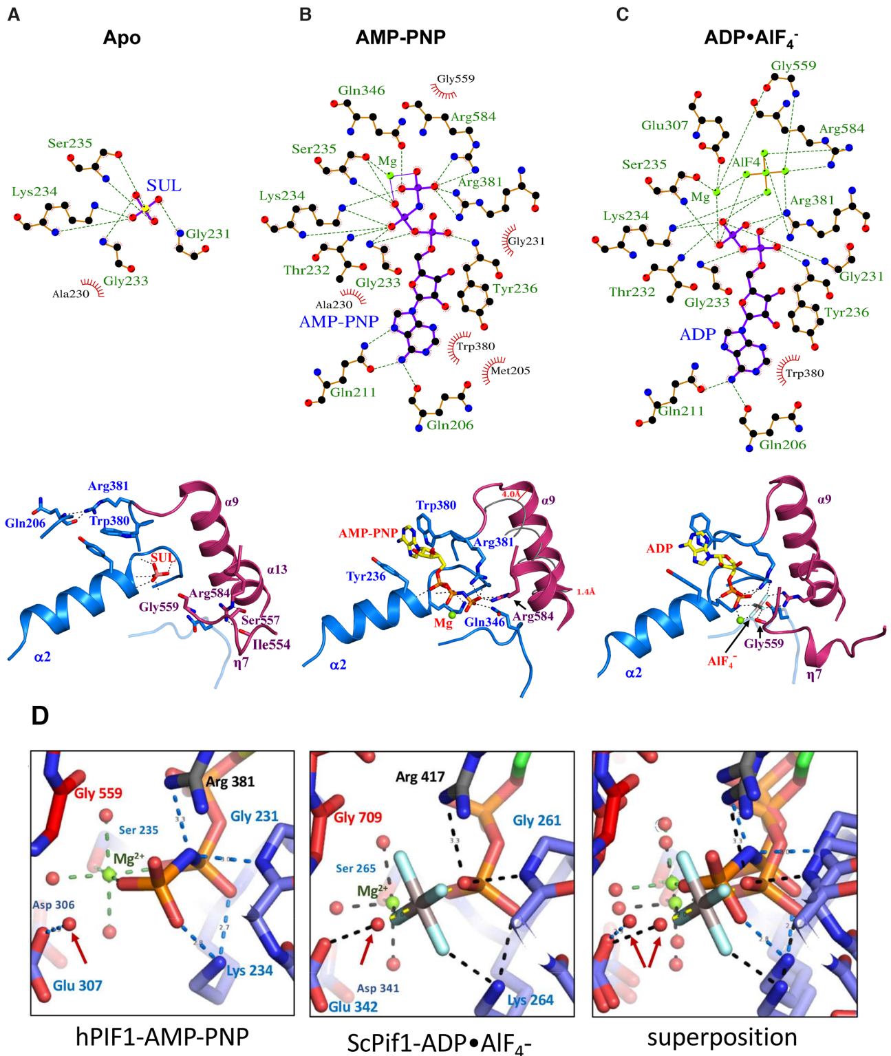
Figure 2. Nucleotide binding and conformational changes in hPIF1. (A) LIGPLOT (45) scheme (above) and structural representation of critical interactions (below) at the nucleotide binding site of apo hPIF1. The green dashed lines represent hydrogen bonds and the non-ligand residues involved in hydrophobic contacts are indicated with annotations in red. Note, the sulphate ion is coordinated at the position of the ATP \beta -phosphate. (B) and (C), as in (A) for the AMP-PNP and ADP•AlF 4 - bound hPIF1 structures. In (B), centre, the conformation of the \alpha 9 helix in apo hPIF1 is represented by a grey tube and the relative displacement is indicated. (D) A comparison of the ATP binding site in hPIF1-AMP-PNP (left), ScPif1-ADP•AlF 4 - (centre) and the superposition of the two (right). The attacking water is indicated with an arrow in each case.
