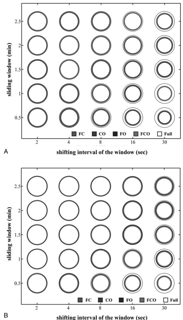
Figure 4. The presentation of accuracy rate for variant spatial areas under N 10 scaling. The spatial location of detected area is shown in circles for (A) artificial neural network and (B) support vector machine, presented with accuracy rate. Within each graph, different combinations of electroencephalography channels are demonstrated in FC combination in light gray area (referring to F3, F4, C3, C4), CO combination in dark gray area (referring to C3, C4, O1, O2), FO combination in black area (referring to F3, F4, O1, O2) and FCO combination in extra-light gray area (referring to all channels, F3, F4, C3, C4, O1, O2). Here, 100% of accuracy rate is denoted as “Full” with a dark line.
