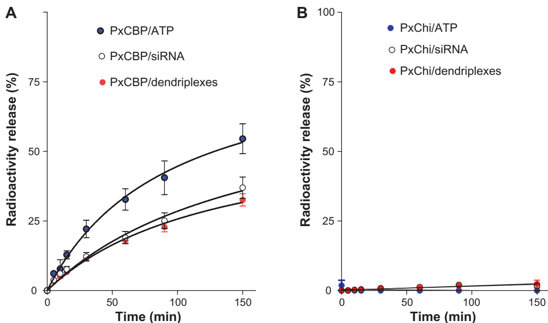
Figure 4 Release profile of radioactivity from in situ-forming (A) poloxamer/carbopol and (B) poloxamer/chitosan gels as function of time.
