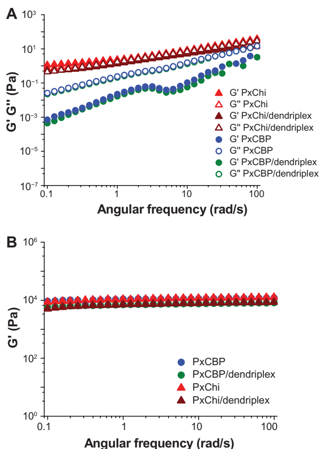
Figure 3 Elastic ( G' ) and viscous ( G'' ) modulus as a function of angular frequency of in situ-forming gels with or without dendriplexes at (A) 10°C and (B) 25°C. Abbreviations: PxCBP, poloxamer/carbopol gel; PxCChi, poloxamer/chitosan gel.
