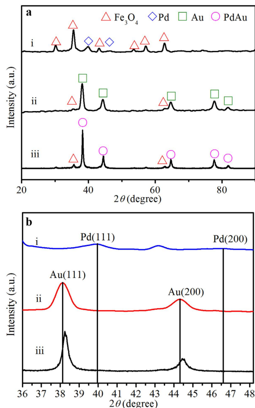
Figure 2. Crystalline structure. (a) XRD patterns of (i) Pd/Fe 3 O 4 , (ii) Au/Fe 3 O 4 and (iii) PdAu/Fe 3 O 4 . (b) Magnification of the peaks (111) and (200) in the 2θ range of 36–48°.
