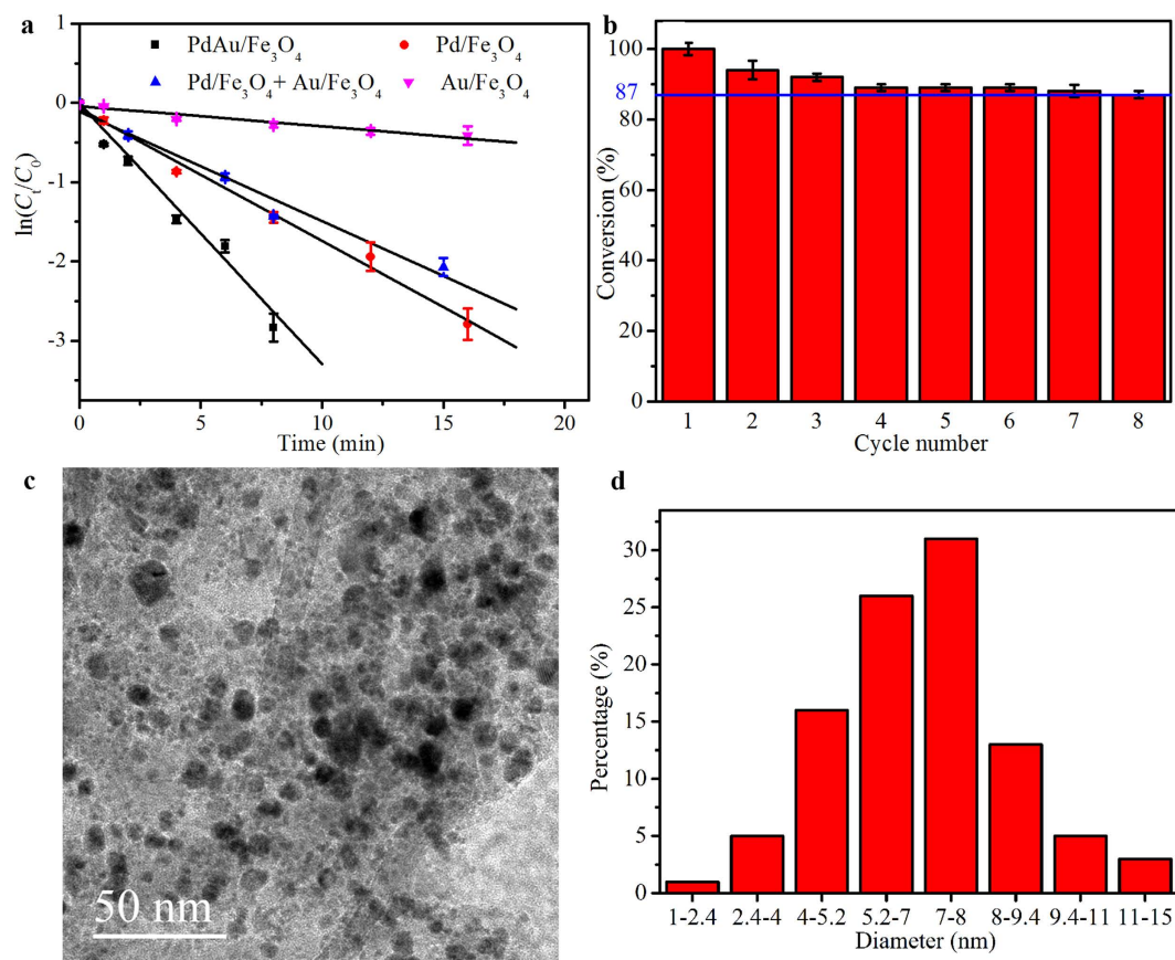
Figure 6. Catalytic performances. (a) Plots of \ln(C_t/C_0) versus time for the reduction of 4-NP by \text{NaBH}_4 in the presence of \text{Pd/Fe}_3\text{O}_4 , \text{Au/Fe}_3\text{O}_4 , \text{Pd/Fe}_3\text{O}_4 + \text{Au/Fe}_3\text{O}_4 or \text{PdAu/Fe}_3\text{O}_4 . (b) The reusability of \text{PdAu/Fe}_3\text{O}_4 as catalyst for reduction of 4-NP by \text{NaBH}_4 . (c,d) TEM image and size distribution of \text{PdAu/Fe}_3\text{O}_4 after reusing for eight runs. Error bars represented standard deviation ( n = 3 ). Significant differences based on the one-way ANOVA ( p < 0.05 ).
