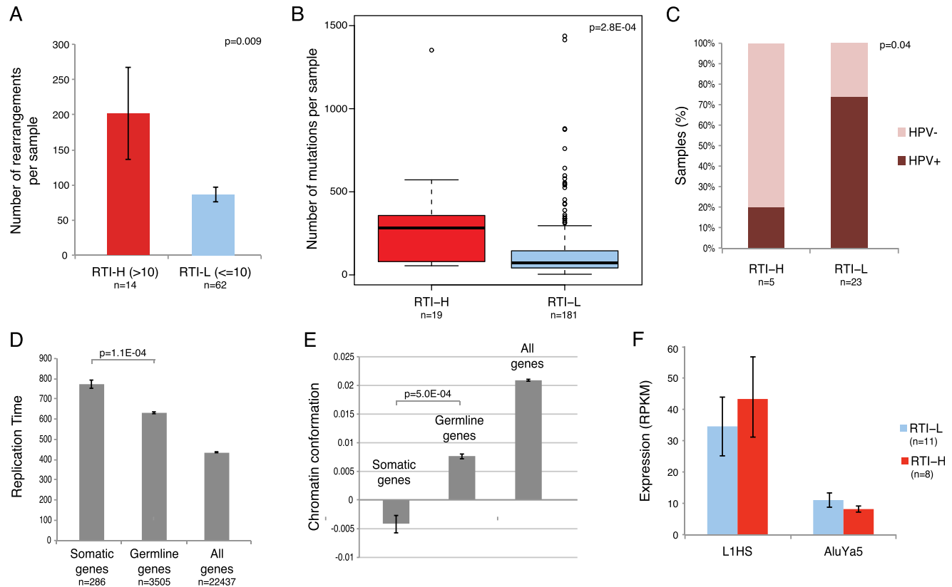
Figure 4. Retrotransposon load is correlated with genomic instability, late-replication, and closed chromatin. (A) Number of somatic rearrangements in LUSC, LUAD, and HNSC samples with high retrotransposon load (>10 somatic retrotransposon insertions, RTI-H) and with low retrotransposon load ( \leq 10 somatic insertion, RTI-L). (B) Number of somatic mutations in RTI-H and RTI-L samples across all 11 tumor types. (C) HPV status of RTI-H and RTI-L HNSC samples. (D) Replication timing of genes that contain somatic retrotransposon insertions versus genes that contain germline insertions, and all RefSeq genes. Later replicating genes have higher values of replication time on the y-axis. (E) Chromatin conformation of genes that contain somatic retrotransposon insertions versus genes that contain germline insertions, and all RefSeq genes. The y-scale represents relative chromatin "openness," the lower the y-value, the more closed the chromatin state. (F) Expression (RPKM) of consensus L1HS and AluYa5 sequences in RTI-H and RTI-L LUSC samples. All error bars represent standard error of the distribution.
