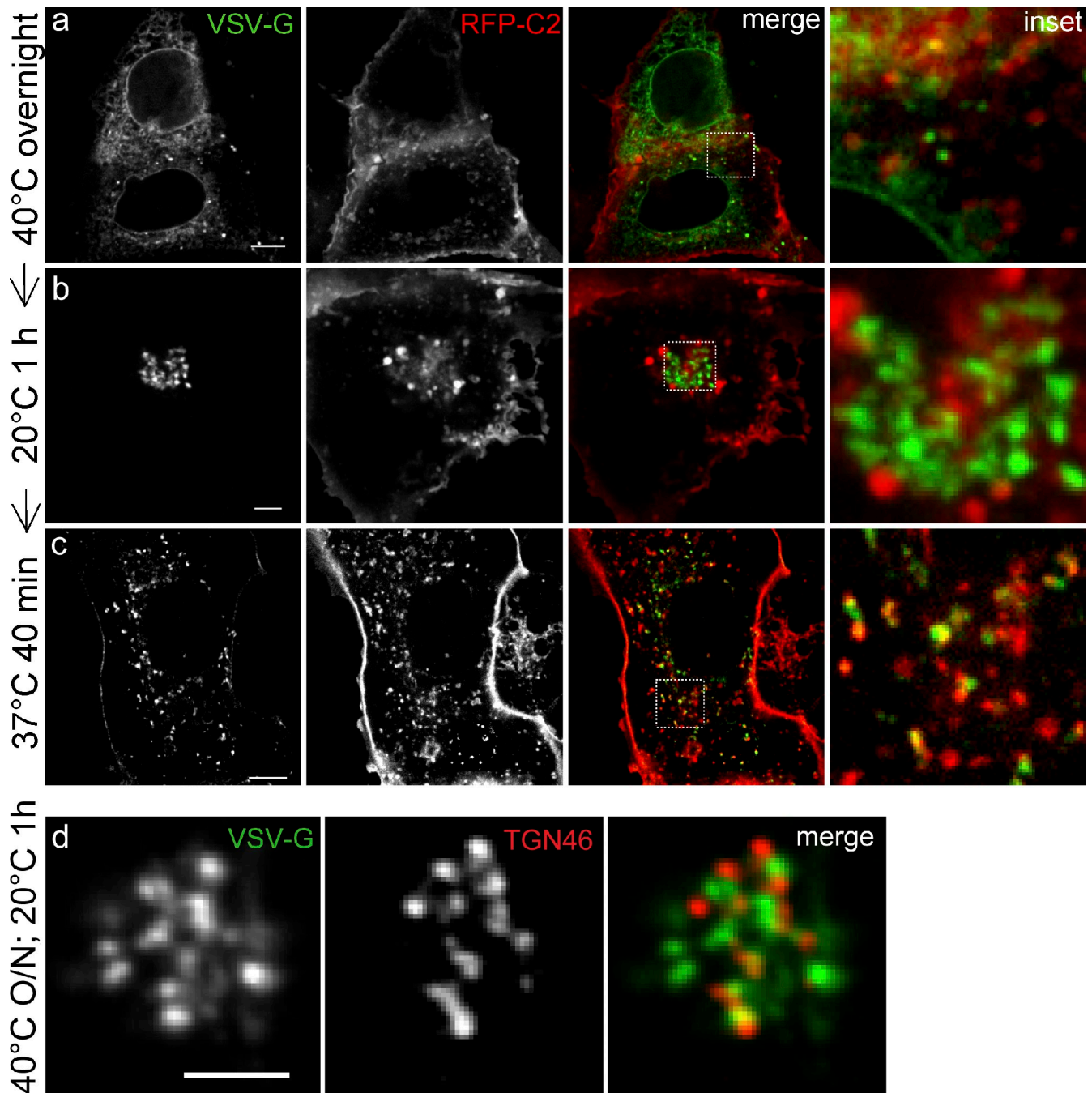
Figure 8. PS becomes cytosolically exposed during progression through the secretory pathway. COS7 were cells double-transfected with VSVG-GFP and mRFP-Lact-C2 (a–c), then incubated as indicated to label the ER (40°C overnight), the Golgi complex (20°C for 1 h after 40°C overnight), and post-Golgi compartments (37°C for 40 min, after 40°C overnight followed by 1 h at 20°C). Insets show enlargement of indicated merged image. Cells expressing VSVG-GFP (d) were grown overnight at 40°C, then shifted to 20°C for 1 h, fixed, and immunostained for TGN46. Insets show enlarged views of the boxed region in the merged image. Bars, 5 \mu m.
