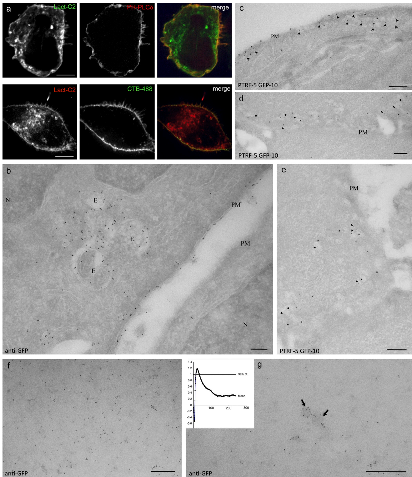
Figure 1. Plasma membrane localization of expressed GFP-Lact-C2. (a, top) A431 cells cotransfected with GFP-Lact-C2 (left) and RFP-PH-PLC \delta (middle), as well as a merged image (right). (a, bottom) A431 cells transfected with mRFP-Lact-C2 and stained with Alexa Fluor 488-labeled cholera Toxin B. (b) Representative frozen section of cells expressing GFP-Lact-C2 and immunogold labeled for the GFP tag. Note labeling over the PM of the expressing cell, but not the neighboring cell, and the lack of cytosolic labeling. The nucleus (N) and nuclear envelope are unlabeled but multivesicular endosomes (E) show significant labeling. (c–e) Cells transfected with GFP-Lact-C2 double labeled for PTRF/cavin-1 (small gold) and GFP (large gold). Note the significant labeling for GFP in the regions enriched in PTRF/cavin-1-labeled caveolae (arrowheads). (f and g) PM lawns were prepared from GFP-Lact-C2-transfected cells and labeled with anti-GFP antibody gold conjugates. GFP-Lact-C2 is clustered in undifferentiated regions of the PM (f) and also labels vesicular profiles (g). Arrows indicate membrane domains consistent with caveolae. Cluster analysis suggests peak clustering at \sim 22 nm (inset). Bars: (b–g) 200 nm.
