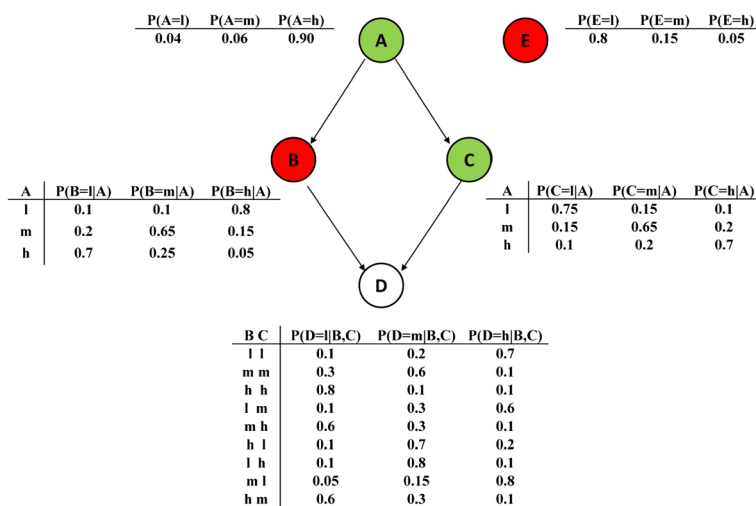
Fig. 1 Illustrative Bayesian network describing causal relationships between five variables, with their associated conditional probability tables. The values of each variable have been discretized into low (l), medium (m) and high (h) bins. The notation P(B=l|A) refers to the probability of B being in the low value bin, conditional upon the value of A (which itself can be l, m or h). Note that with one parent only (i.e. the case for nodes B and C), both row and column probabilities sum to 1, whereas with multiple inputs (i.e. in the case of D), only the rows sum to 1. The nodes are colored green (high), white (medium) and red (low) to illustrate in silico perturbation where A falls into a high concentration bin (probability 0.9) and E falls into a low concentration bin (probability 0.8). The implications of this are demonstrated through the conditional probability tables associated with each downstream node wherein having D in a given concentration state is dictated by the particular combination of states of its parents B and C as dictated by their corresponding overall (marginal) probabilities (the entries as captured in the conditional probability tables do not change on intervention), as summarized in the histogram attached to each node. Note that the overall marginal probability of D being in a particular state (which changes under intervention) is the sum as summarized in the histogram attached to each node. Readers more familiar with Bayesian networks will note that the sub-network structures (B \rightarrow A, A \rightarrow C, B \rightarrow D, C \rightarrow D) and (C \rightarrow A, A \rightarrow B, B \rightarrow D, C \rightarrow D) are both Markov equivalent with the present one (A \rightarrow B, A \rightarrow C, B \rightarrow D, C \rightarrow D) . When we condition on A, the other nodes B and C become independent no matter whether A is a tail-to-head or tail-to-tail intermediate node (this scenario differs from that seen with head-to-head node D). In other words, these three sub-networks specify the same independent assumptions belonging to the same equivalence class and the true causal network can possibly be any one of the sub-network solutions. However, causal networks based on observation alone (i.e. without intervention, which is an important tool for inferring causality) can be still partially constructed. In the present study, prior knowledge seed network edge directionalities were assigned by a modified depth-first search algorithm which helped to choose the sub-network from an equivalence class containing more than one Markov equivalent member as suggested here (see later)
