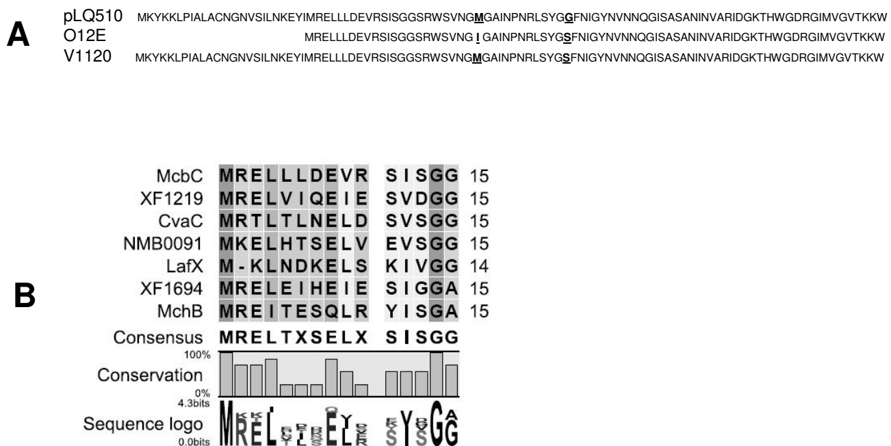
Figure 2 Putative bacteriocin proteins encoded by the mcb locus. (A) Amino acid sequence of the predicted McbC proteins encoded by the mcb locus in plasmid pLQ510, M. catarrhalis O12E, and M. catarrhalis V1120. Residues that differ among the proteins are underlined and bolded. (B) Alignment of the amino acid sequence of the putative leader of the M. catarrhalis O12E McbC protein with that of leader peptides of proven and hypothetical double-glycine peptides from other bacteria including CvaC [GenBank: CAA11514 ] and MchB [GenBank: CAD56170 ] of E. coli , NMB0091 [GenBank: NP_273152 ] of Neisseria meningitidis , XF1219 [GenBank: AAF84029 ] and XF1694 [GenBank: AF84503 ] of Xylella fastidiosa and LafX [GenBank: AAS08589 ] of Lactobacillus johnsonii . Highly conserved amino acids are shaded with dark grey. This latter figure is adapted from that published by Michiels et al [30].
