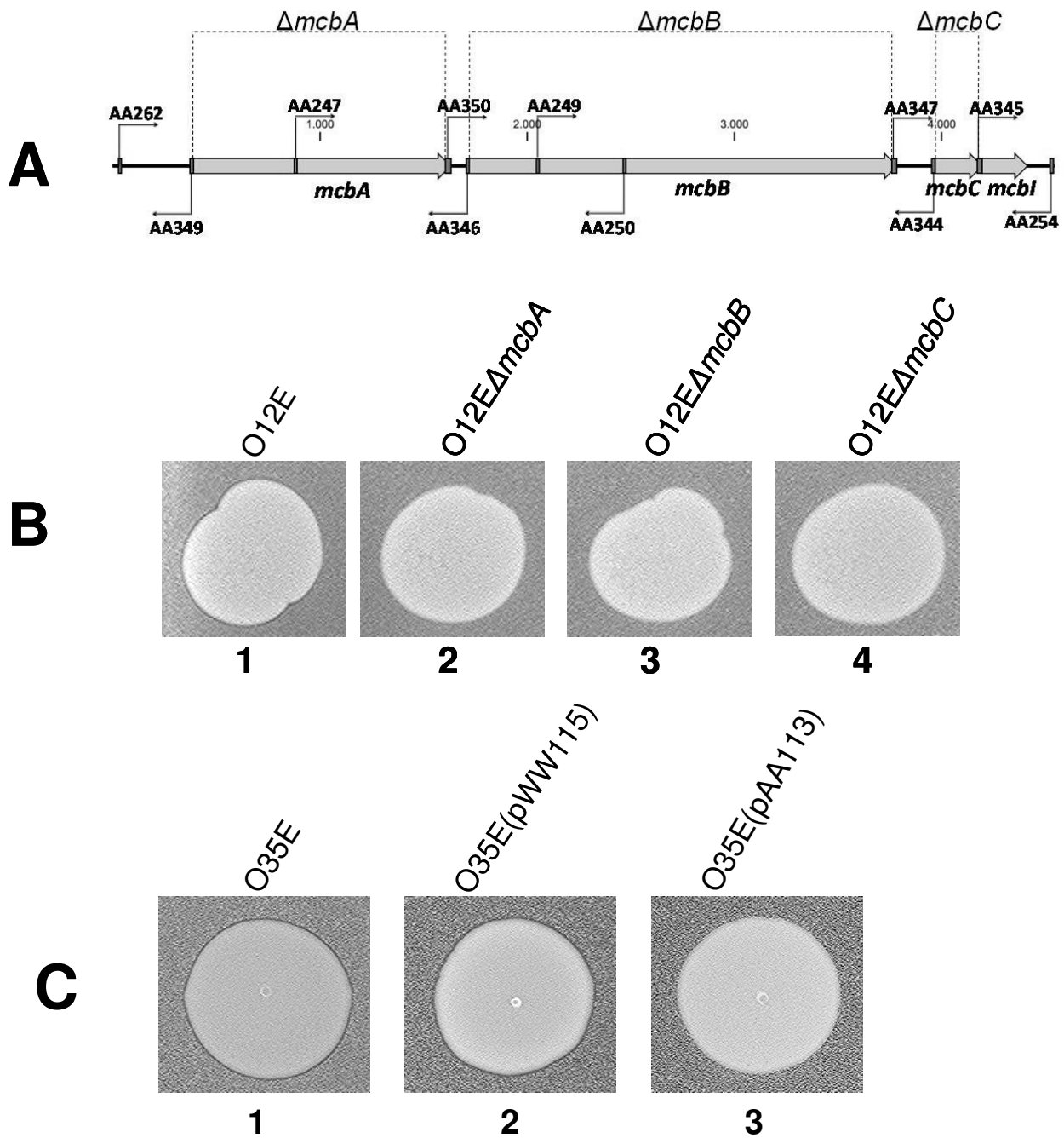
Figure 5 Analysis of mutant and recombinant M. catarrhalis strains. (A) Schematic showing the mcbABC locus in the O12E chromosome and the position of the oligonucleotide primers used to construct the three different in-frame deletion mutations in this locus. The extent of the deletion in each ORF is indicated. (B) Bacteriocin production assay using O35E as the indicator strain together with the following test strains: panel 1, O12E; panel 2, O12EΔ mcbA ; panel 3, O12EΔ mcbB ; panel 4, O12EΔ mcbC . Panel C, Use of recombinant M. catarrhalis strains to demonstrate that expression of McbI in O35E confers protection against killing by strain O12E. M. catarrhalis O12E was used as the test strain in a bacteriocin production assay with three different M. catarrhalis strains as the indicator. Panels: A, O35E wild-type; B, O35E(pWW115) [vector-only control]; C, O35E(pAA113) [expressing McbI ].
