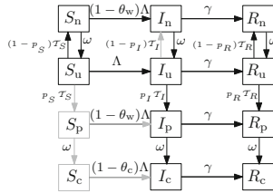
Fig. 1 Flowchart of the SIR (Susceptible-Infectious-Recovered) model, A1. The disease-based status of a compartment X ( X \in \{S, I, R\} ) is combined with the testing status including X_u, X_p, X_n and X_c , for untested , waiting-for-positive , waiting-for-negative , or confirmed positive , respectively. The force of infection is denoted by \Lambda (Eq. 3); \gamma is the recovery rate; \omega is the rate of test return; and \mathcal{T}_X (Eq. 2) and p_X represent the per capita testing rate and the sensitivity (probability that an infected individual tests positive), respectively, for compartment X . For further description of the parameters see Table 1. Note that there is a slight mismatch in the top-to-bottom order of the testing-based compartments of each disease-based compartment X between this flowchart and the model equations (A1); here we have switched X_u and X_n for visual clarity
