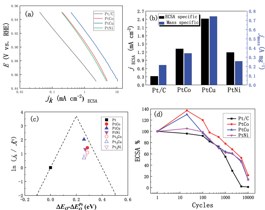
Fig. 8 (a) ECSA specific kinetic current densities ( j_k ) for mesoporous PtM (M = Co, Cu, Ni) and Pt/C catalysts. (b) The ECSA and Pt mass specific kinetic current densities for mesoporous PtM and Pt/C catalysts at 0.90 V (vs. RHE). (c) Volcano plots for the oxygen reduction reaction on mesoporous PtM (M = Co, Cu, Ni) alloys. (The measured experimental data are marked by solid symbols and the data from literature 29,37 are marked by hollow symbols. The dash lines are the theoretical predictions. 51,52 ) (d) The loss of ECSA for mesoporous PtM and Pt/C catalysts vs. the scanning cycles in N 2 -purged 0.1 M HClO 4 solution (0.05–1.4 V vs. RHE, scan rate: 50 mV s -1 ).
