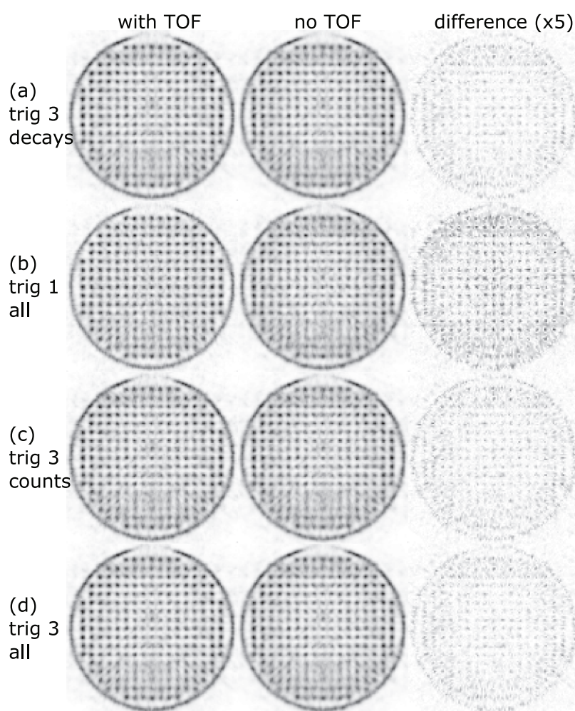
Figure 11. Transversal slices through the reconstructed rabbit-sized phantom. The voxel pitch is 1 mm, and the slice thickness is 10 mm. The complete datasets of trig 1 and trig 3 (all) are truncated for comparison: trig 3 decays matches trig 1 all in terms of the number of tracer decays and trig 3 counts matches trig 1 all in terms of the number of coincidences (table 4). The third column shows the absolute difference multiplied by a factor of 5 between the two reconstructions for each measurement.
