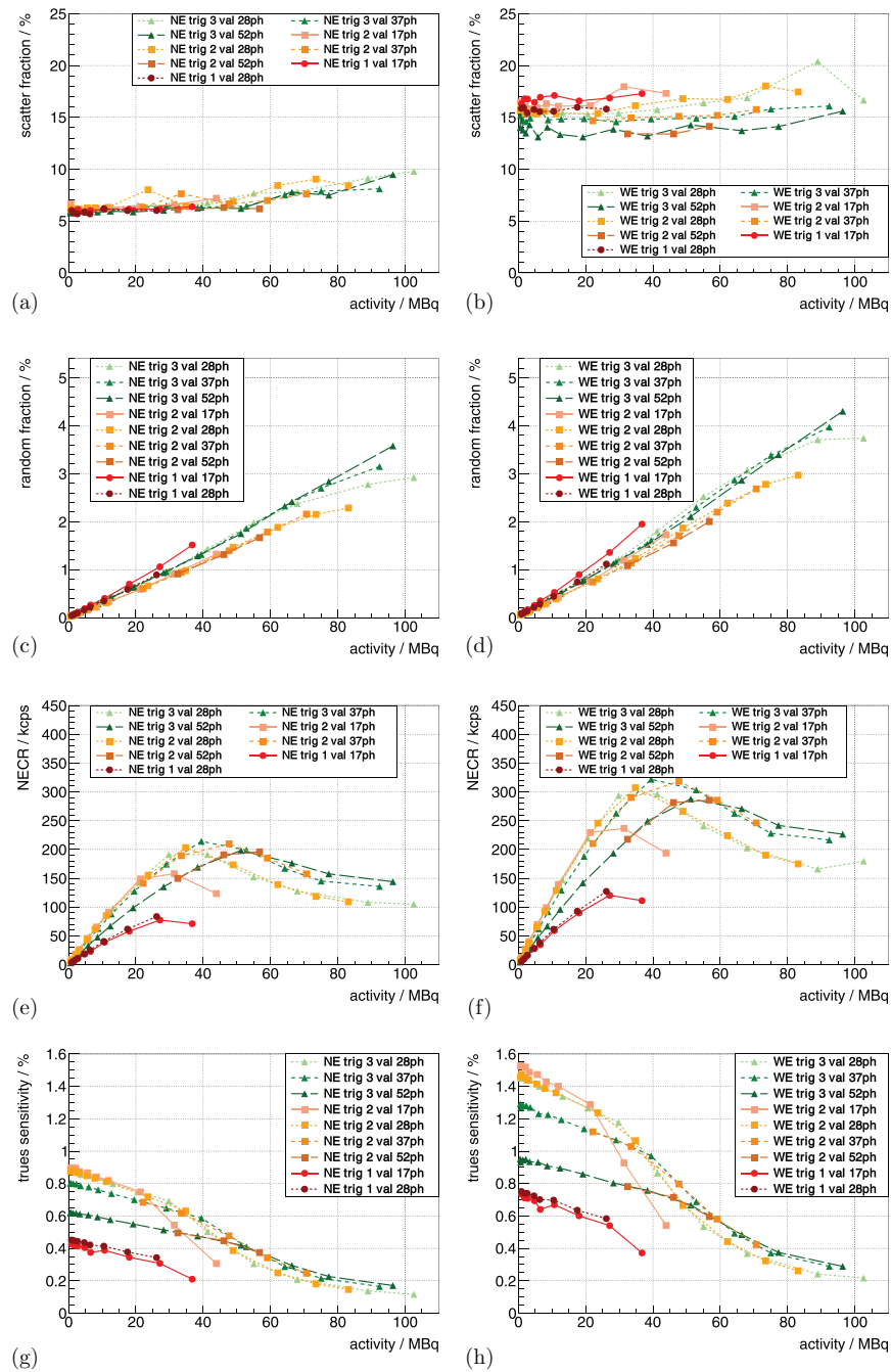
Figure 8. (a) and (b) show the scatter fraction curves for the mouse-sized scatter phantom for a constant V_{ov} = 2.5 \text{ V} and T_C = 0^\circ\text{C} for different trig and val. The two bands for the different energy windows can clearly be distinguished. For the same measurement, (c) and (d) show the random fraction, (e) and (f) the NECR curves and (g) and (h) the trues sensitivity.
