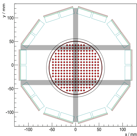
Figure 13. Transversal cross section through the gantry. The LYSO crystal array outlines are drawn in light blue, and the light guide in green; the sensor tile is sketched in red. The rabbit-sized phantom is shown at the measured untilted position, which is not centered along the y -axis. The gaps in the horizontal and vertical direction are plotted in gray, parallel to the symmetry axes of the Cartesian grid of the phantom and intersecting the activity distribution.
