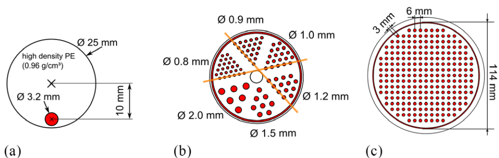
Figure 3. (a) A slice through the mouse-sized scatter phantom; the scatter phantom has an axial extent of 70 mm. (b) Hot-rod phantom used to investigate the spatial resolution; the structured region has a diameter of 28 mm, and the evaluated profiles are marked in orange. (c) Rabbit-sized phantom used to investigate the benefit of TOF information for image reconstruction; the structured part of the phantoms (b) and (c), for which the slices are shown, have an axial extent of 20 mm, and the FDG-filled areas are marked in red.
