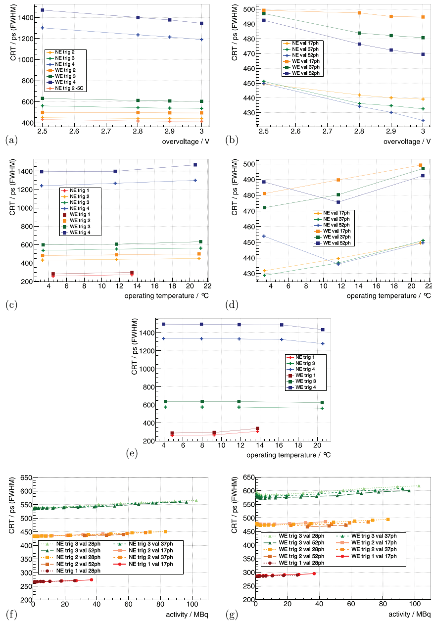
Figure 6. The CRT measured with the ^{22}\text{Na} point sources is shown in (a) as a function of V_{ov} for different trig and in (b) for different val. It is shown for a constant V_{bias} as a function of T_{op} in (c) for different trig and in (d) for different val. For a constant V_{ov} , it is shown as a function of T_{op} in (e) for different trig. Measured with the FDG-filled scatter phantom, it is shown in (f) and (g) as a function of activity for different trig and val. (a) T_C = 15^\circ\text{C} , val | 7ph. (b) T_C = 15^\circ\text{C} , trig 2. (c) const V_{bias} , V_{ov}(T_C = 15^\circ\text{C}) = 2.5\text{ V} , val | 7ph. (d) const V_{bias} , V_{ov}(T_C = 15^\circ\text{C}) = 2.5\text{ V} , trig 2. (e) const V_{ov}(T_C) = 2.5\text{ V} , val | 7ph. (f) T_C = 0^\circ\text{C} , V_{ov} = 2.5\text{ V} . (g) T_C = 0^\circ\text{C} , V_{ov} = 2.5\text{ V} .
