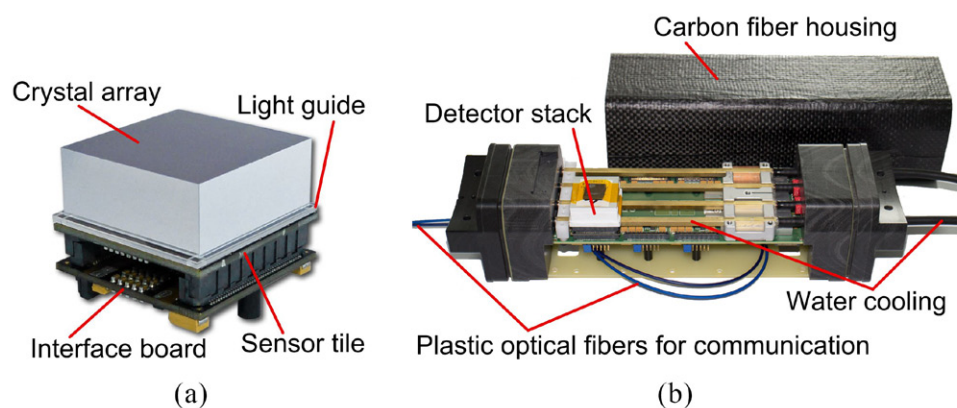
Figure 1. (a) The detector stack consists of an interface board, the sensor tile and a pixelated scintillating crystal array mounted on a light guide (© [2012] IEEE. Reprinted, with permission, from Weessler et al (2012)). (b) The singles detection module is able to house up to six stacks. Only one detector stack is mounted to reveal the cooling pipes (reprinted from Wehner et al (2014)).
