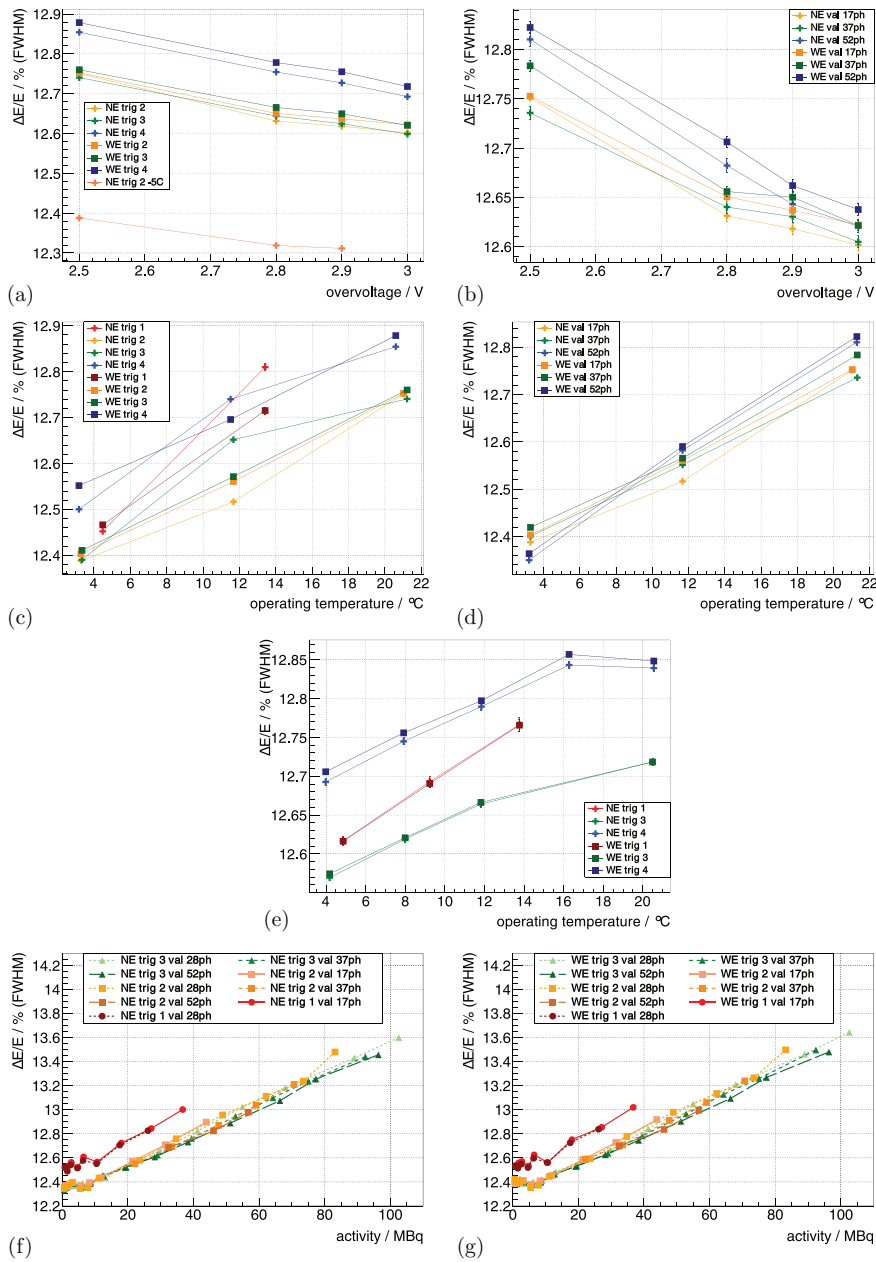
Figure 5. \Delta E/E of the whole insert measured with the ^{22}\text{Na} point sources is shown as a function of V_{ov} in (a) for different trig and in (b) for different val. It is then shown as a function of T_{op} for a constant V_{bias} in (c) for different trig and in (d) for different val. For a constant V_{ov} , it is shown as a function of T_{op} in (e) for different trig. Measured with the FDG-filled scatter phantom, it is shown in (f) and (g) as a function of activity for different trig and val. (a) T_C = 15^\circ\text{C} , val | 7ph. (b) T_C = 15^\circ\text{C} , trig 2. (c) const V_{bias} , V_{ov}(T_C = 15^\circ\text{C}) = 2.5\text{ V} , val | 7ph. (d) const V_{bias} , V_{ov}(T_C = 15^\circ\text{C}) = 2.5\text{ V} , trig 2. (e) const V_{ov}(T_C = 15^\circ\text{C}) = 2.5\text{ V} , val | 7ph. (f) T_C = 0^\circ\text{C} , V_{ov} = 2.5\text{ V} . (g) T_C = 0^\circ\text{C} , V_{ov} = 2.5\text{ V} .
