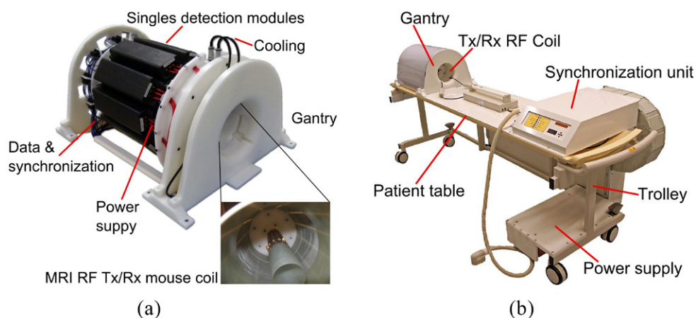
Figure 2. (a) The gantry of the PET insert holds ten SDMs (© [2012] IEEE. Reprinted, with permission, from Weessler et al (2012)). (b) The gantry, a synchronization unit and a power supply are mounted on a trolley allowing easy insertion into an MRI scanner. Only a single data link, a power cable and the cooling tubes have to be connected.
