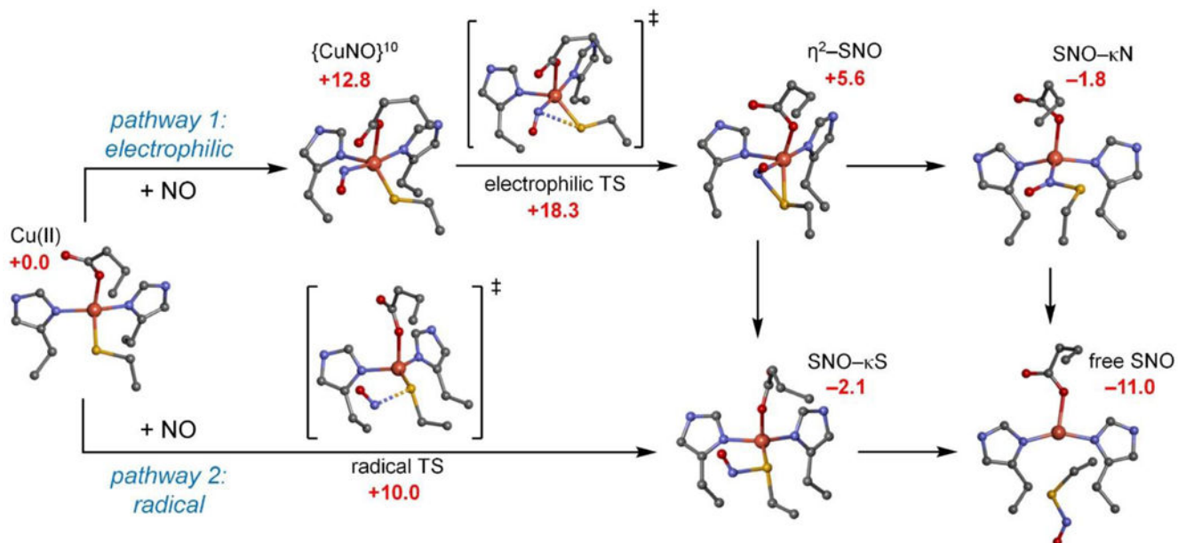
Figure 3. Electrophilic and radical pathways for (Cys)S-NO bond formation and possible isomers of the Cu(I)/(Cys)S-NO product
