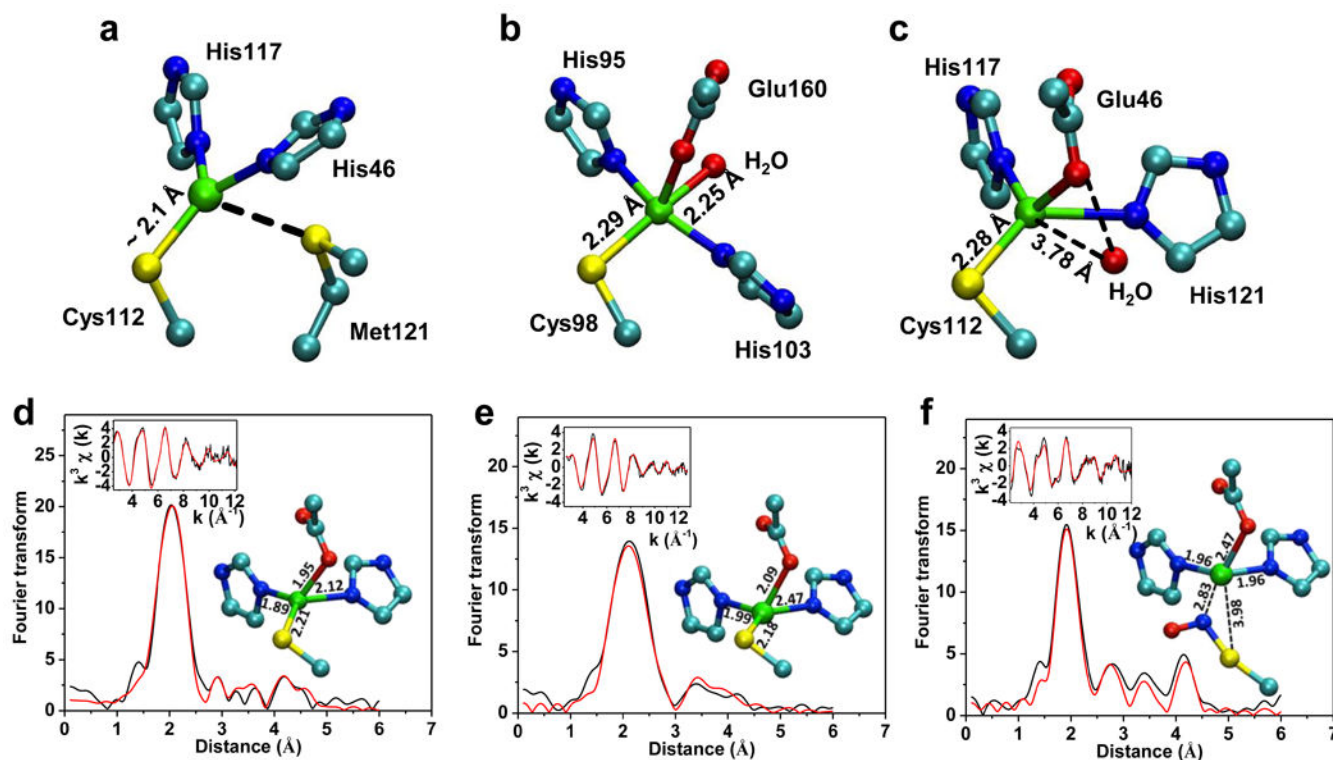
Figure 1. Geometries of Cu(II) binding sites and Fourier transform of EXAFS data with fitting a , WTaz (PDB: 4AZU), b , nitrosocyanin (PDB: 1IBY) and c , M121H/H46EAz (PDB: 4WKX). The Cu(II)-binding site in Cu(II)-M121H/H46EAz adopted a more distorted tetrahedral geometry compared to WTaz. The Cu-S(Cys112) distance in Cu(II)-M121H/H46EAz was 2.28 Å, longer than the ~2.1 Å in blue copper proteins, but comparable to that in nitrosocyanin (2.29 Å). An exogenous water was at 3.78 Å from the Cu(II) within hydrogen bonding distance of the coordinating O of Glu46 (2.56 Å) in Cu(II)-M121H/H46EAz. Fourier transform and EXAFS (inset) for d , Cu(II)-M121H/H46E/F114PAz, e , Cu(I)-M121H/H46E/F114PAz and f , NO treated Cu(II)-M121H/H46E/F114PAz. The NO treated Cu(II)-M121H/H46E/F114PAz has different EXAFS pattern from Cu(I)-M121H/H46E/F114PAz, indicating the process was not simple reduction from Cu(II) to Cu(I). The NO treated Cu(II)-M121H/H46E/F114PAz was best fitted when the Cys ligand was moved to 3.98 Å and a new N ligand was added at 2.83 Å, suggesting that the weak interaction between Cu(I) and S-nitrosothiol is through the N-atom. Experimental data are shown as solid black lines, and the simulations as red lines. Copper atoms are green; oxygen atoms are red; sulfur atoms are yellow; nitrogen atoms are blue; carbon atoms are cyan.
