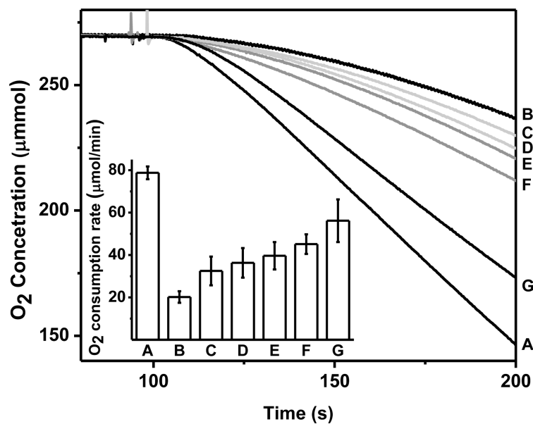
Figure 4. Effect of Cu(II)-M121H/H46E/F114PAz on NO inhibition of E. coli cytochrome bo 3 oxidase
