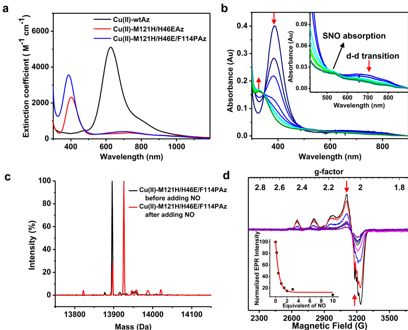
Figure 2. UV-Vis absorption, Mass spectrometric and EPR spectroscopic characterization of S-nitrosylation in engineered red copper protein a , The UV-Vis spectra of Cu(II)-WTaz, Cu(II)-M121H/H46EAz and Cu(II)-M121H/H46E/F114PAz. The S(Cys) \rightarrow Cu(II) LMCT band of Cu(II)-M121H/H46E/F114PAz was at 390 nm, blue shifted compared to WTaz, but identical to nitrosocyanin. b , Kinetic UV-Vis spectra of 110 \mu M Cu(II)-M121H/H46E/F114PAz reacting with 1 equivalent of DEA NONOate in 50 mM Mes buffer at pH 6. A spectrum was recorded every 10 s. Upon NO addition, immediate bleaching of the 390 nm peak and an isosbestic point at 347 nm were observed. c , ESI-MS before (black) and after (red) NONOate addition. A mass increase of +29 Da compared to apo-M121H/H46E/F114PAz supports S-nitrosylation of the protein. d , X-band EPR spectra of Cu(II)-M121H/H46E/F114PAz reacting with different amounts of NO. Inset: EPR integration as a function of NO equivalents. Decreasing signal intensity with increasing concentration of NO indicates the formation of an EPR silent species.
