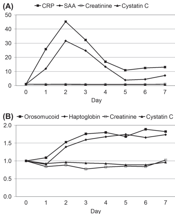
Figure 1. Changes in plasma levels of (A) CRP, SAA, creatinine and cystatin C and of (B) orosomuroid, haptoglobin, creatinine and cystatin C during seven consecutive days after elective surgery. Day zero denotes the day before surgery. The ordinates represent the median level of each analyte in multiples of the preoperative level.
