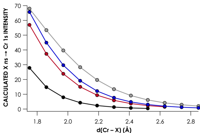
Figure 6. Dependence of the intensity of X ns \rightarrow Cr 1s K\beta'' transitions for the series [\text{Cr}^{\text{III}}(\text{NH}_3)_5\text{X}]^{2+} (X = F (black), Cl (red), Br (blue), and I (gray)) on the Cr–X distance.
