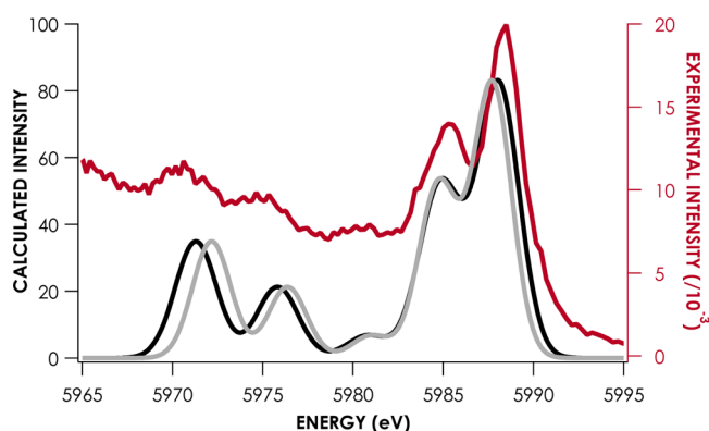
Figure 4. Experimental (red) and BP86/def2-TZVP-ZORA calculated (linear-corrected, black; scalar-shifted, gray) V2C XES spectra for Cp_2Cr .
