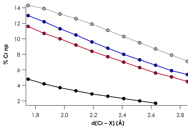
Figure 7. Dependence of the admixture between X valence ns and Cr np for the series [\text{Cr}^{\text{III}}(\text{NH}_3)_5\text{X}]^{2+} (X = F (black), Cl (red), Br (blue), and I (gray)) on the Cr–X distance.
