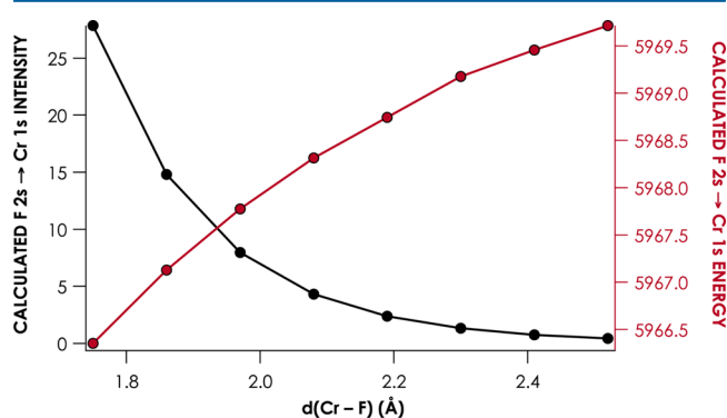
Figure 8. Dependence of the calculated intensity (black) and energy (red) of the F 2s \rightarrow Cr 1s K\beta'' transition for [\text{Cr}^{\text{III}}(\text{NH}_3)_5\text{F}]^{2+} , relative to Cr–X distance.
