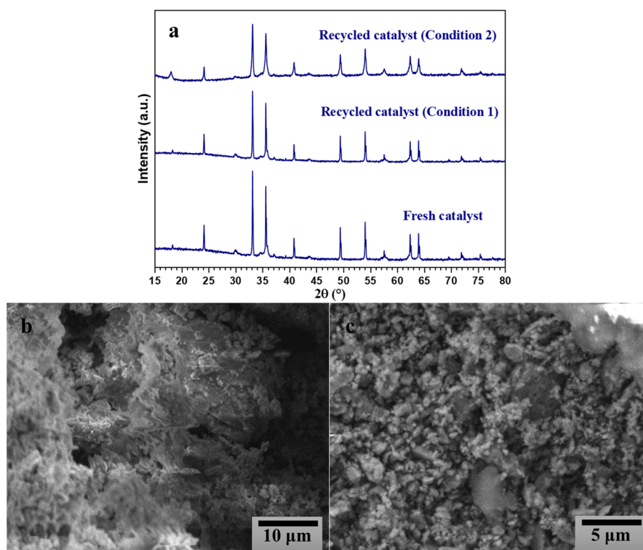
Fig. 13 XRD patterns of the fresh and recycled CuFe 12 O 19 (a), and SEM images of CuFe 12 O 19 after five runs while using (b) tBHP or (c) H 2 O 2 .
