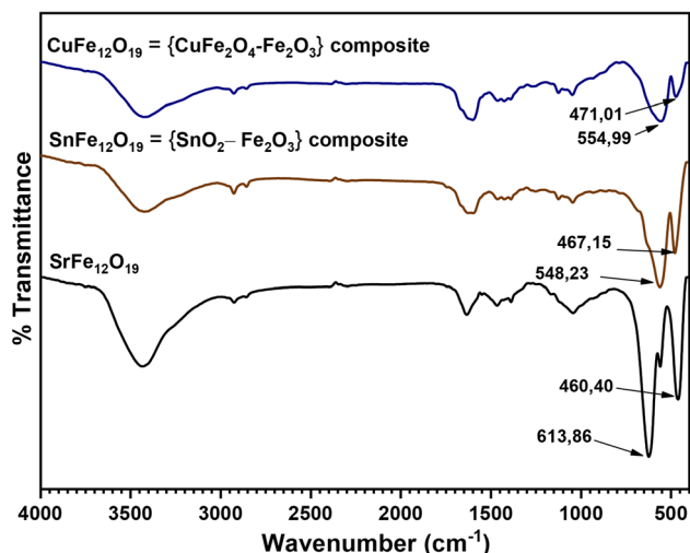
Fig. 3 FTIR spectra of \text{CuFe}_{12}\text{O}_{19} , \text{SnFe}_{12}\text{O}_{19} and \text{SrFe}_{12}\text{O}_{19} .
