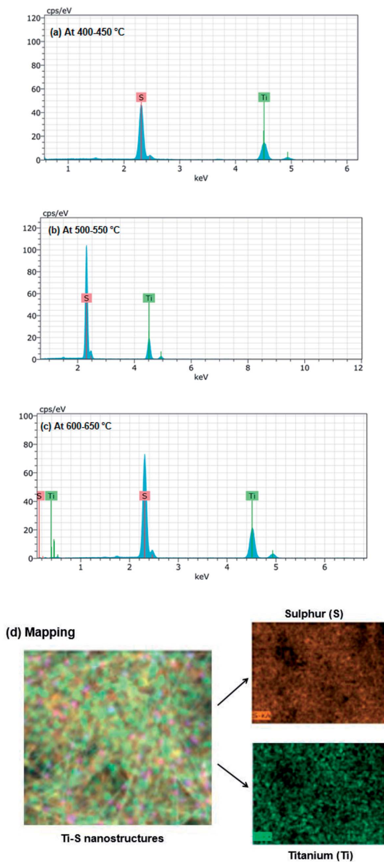
Fig. 4 Energy dispersive X-ray spectrum of titanium sulphide nanostructures grown at different temperature for 24 h (a) 400 °C to 450 °C (b) 500 °C to 550 °C (c) 600 °C to 650 °C (d) EDX elemental mapping of titanium and sulphur.
