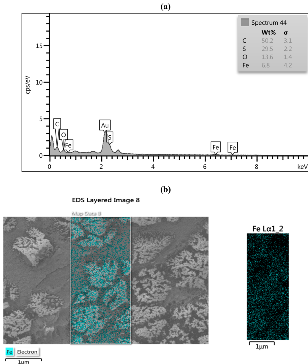
Fig. 3 EDX analysis (a) and (b) elemental mapping of the CMC- g -poly(AA- co -AMPS)/Fe 3 O 4 hydrogel nanocomposite.
