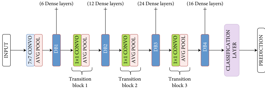
FIGURE 5: DenseNet121 architecture.
