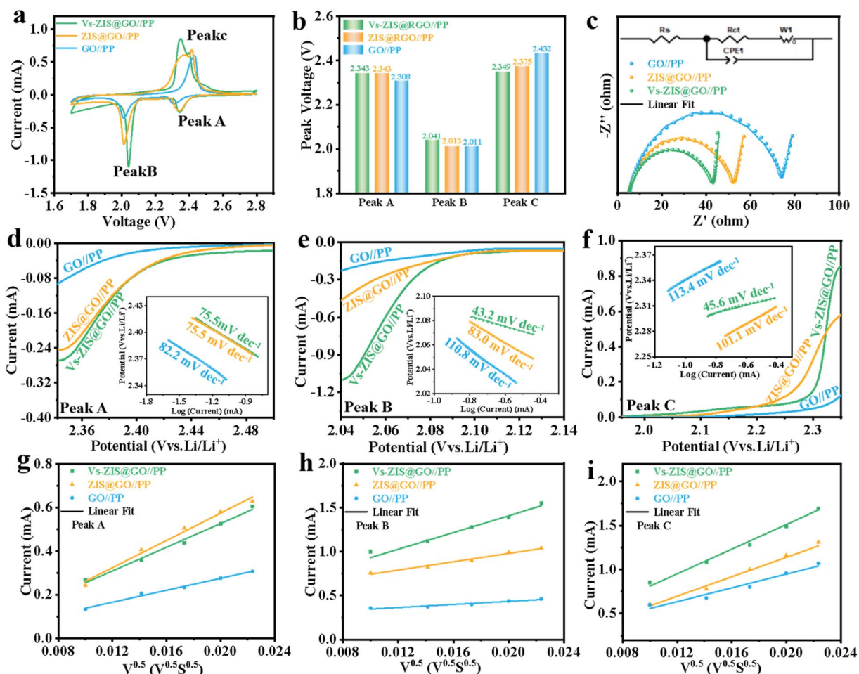
Fig. 5 (a) CV curves, (b) Corresponding peak voltages and (c) EIS of GO//PP, ZIS@RGO//PP and Vs-ZIS@RGO//PP. Potentiostatic polarization curves of GO//PP, ZIS@RGO//PP and Vs-ZIS@RGO//PP at a scan rate of 0.1 \text{ mV s}^{-1} for the (d) Peak A, (e) Peak B and (f) Peak C. The inset shows the corresponding Tafel plots derived from the potentiostatic polarization curves. Plots of CV peak current for the (g) Peak A, (h) Peak B and (i) Peak C versus the square root of the scan rates for the batteries of GO//PP, ZIS@RGO//PP and Vs-ZIS@RGO//PP.
