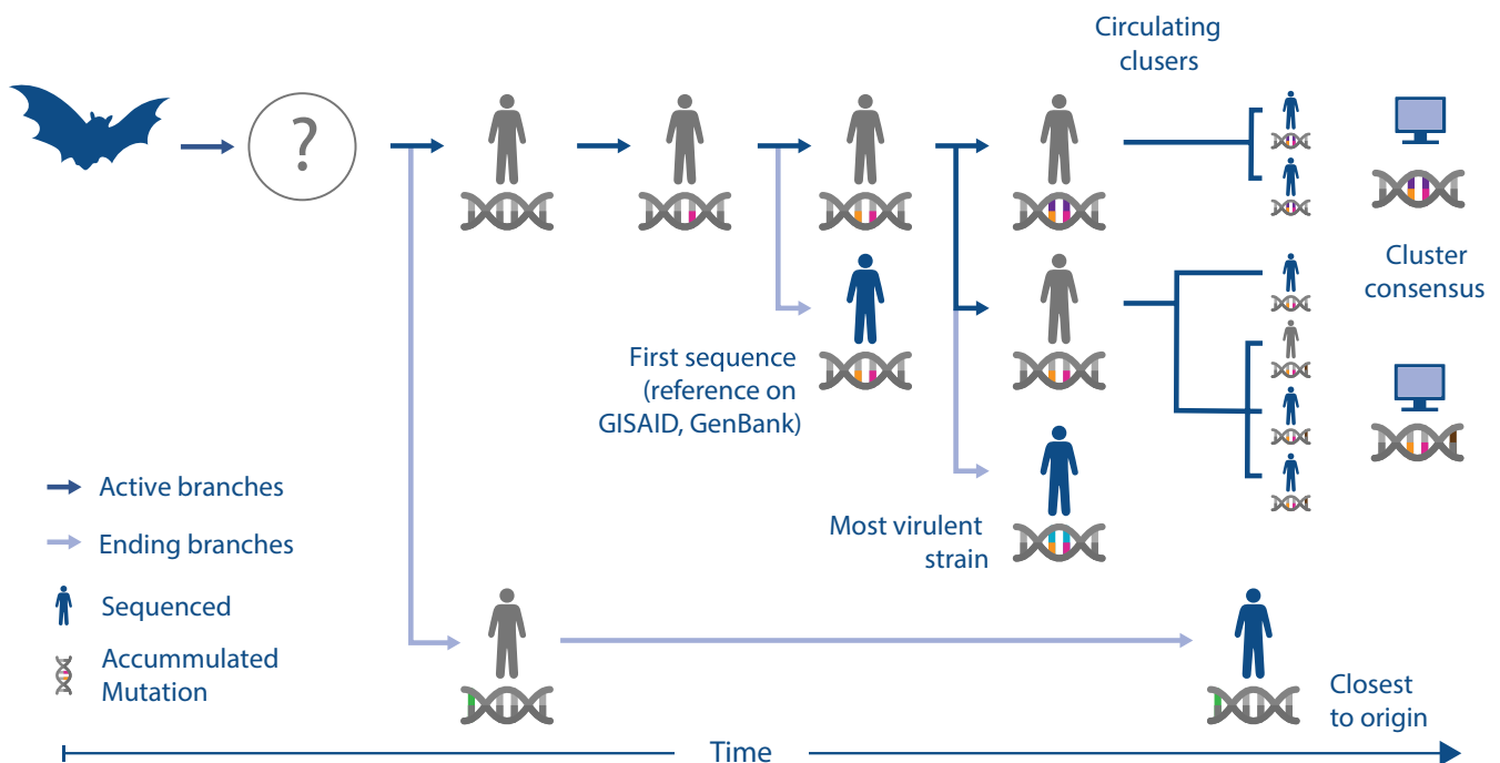
FIGURE 1 Illustration of coronavirus spread while it accumulates mutations. The dark blue arrows represent the main volume of transmissions, while the nucleic acid symbol illustrates mutations acquired by the different viral strains as they enter humans from a primary/reservoir host (represented by the bat symbol) through an intermediate host (which is yet to be identified for SARS-CoV-2). The first human SARS-CoV-2 isolate sequenced (with orange and pink mutation) may not have been the original strain that first infected humans (grey). It is possible that a strain sequenced later (green) may be genetically closer to the original strain. In this scenario, the original strain has not been captured through sequencing at all. It also shows that there may be two currently circulating strains (orange-pink-purple and orange-pink-brown), which in turn might be different from the most virulent one (orange-pink-blue). In the absence of clinical data correlated with SARS-CoV-2 genome isolates, bioinformatic analysis (represented by the computer symbol) can identify clusters and consensus sequences to investigate the genetic diversity of the emerging SARS-CoV-2 strains
