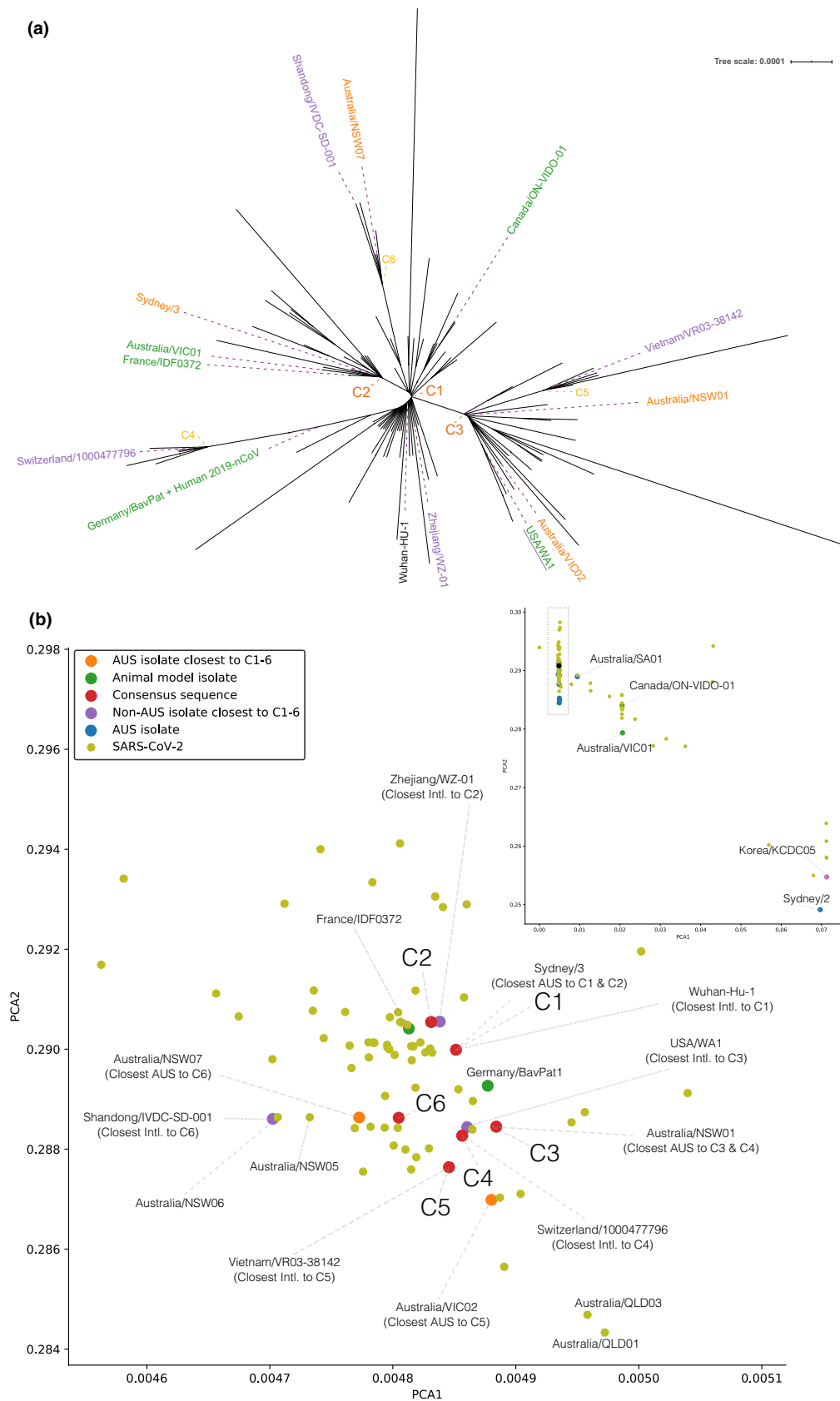
FIGURE 4 Identification of potential viral strains for animal models. Phylogenetic methods (a) show that current animal models (highlighted in green) cover the major clusters (C1-3) but may not capture the emerging clusters. A K-mer based analysis (b) is able to suggest alternative strains that cover all emerging clusters (C4-6). The inset shows the wider region with the main image extent marked by a rectangle
