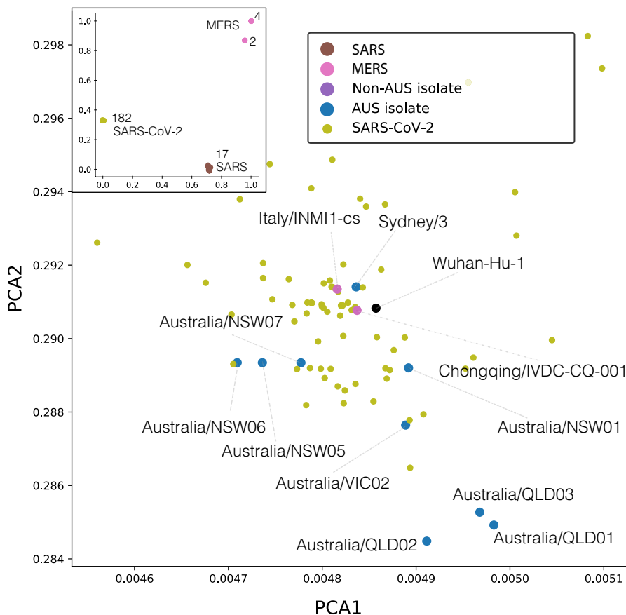
FIGURE 3 PCA plots showing the genomic signatures of different coronavirus sequences. Each point represents the genomic signature for an isolate. Inset Comparison of genomic signatures across different strains of coronavirus. Numbers correspond to the number of isolates at each location. Overall, the genomic signatures for isolates of different coronavirus strains were relatively far apart. Main image Zoomed in PCA plot of the cluster of SARS-CoV-2 isolates, showing the overall genomic signatures of the different strains
