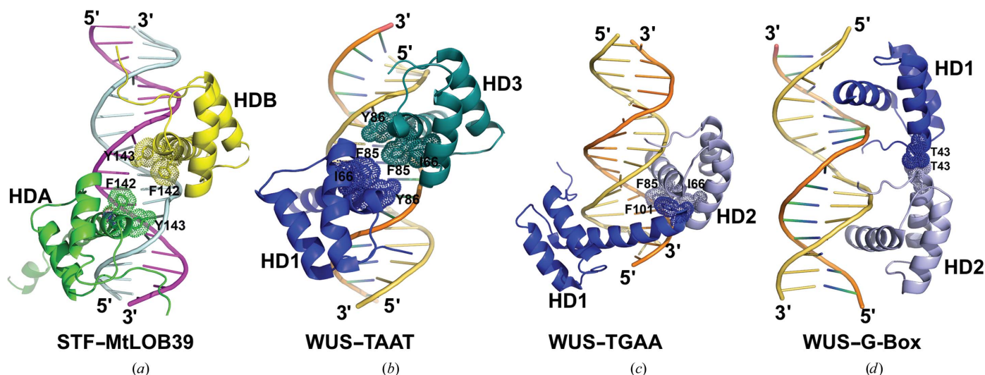
Figure 12 Comparison of DNA binding by STF HDA and HDB with WUS-HD dimers. (a) STF HDA (green) and HDB (yellow). The nonpolar residues buried at the interfaces are shown as sticks, with dotted envelopes indicating the van der Waals radius. STF HDA and HDB are more than 8 Å apart and do not contact each other directly. (b) WUS-HD dimer (blue and teal) bound to the TAAT motif (PDB entry 6ryl). WUS HD1 is bound at the TAAT core, while WUS HD3 is bound at a neighboring location without base-specific interactions. (c) WUS-HD dimer (blue and light blue) bound to the TGAA repeat (PDB entry 6ryd). (d) WUS-HD dimer (blue and light blue) bound to the G-box motif (PDB entry 6ryi).
