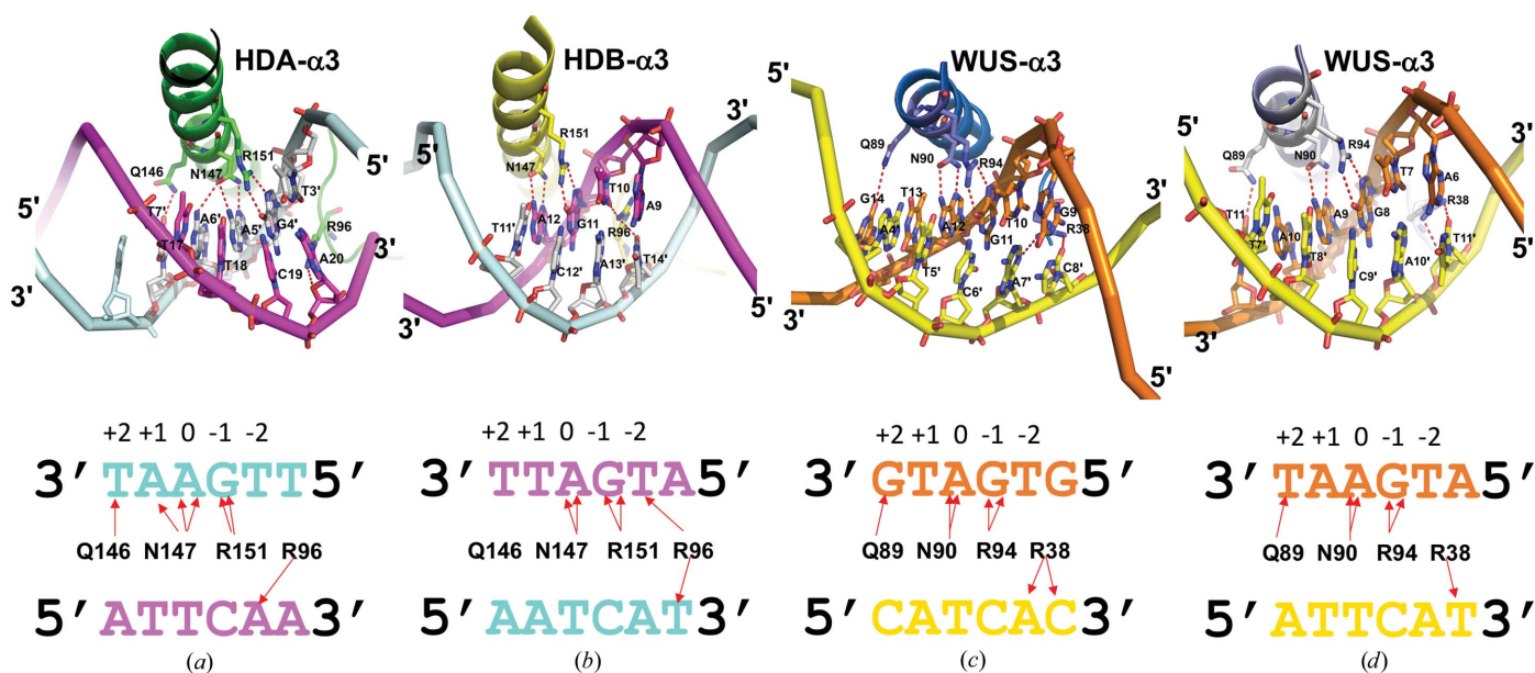
Figure 13 Comparison of major-groove base recognition between STF-HD and WUS-HD. (a) TGA recognition by STF HDA helix \alpha 3 (green). (b) TGA recognition by STF HDB helix \alpha 3 (yellow). (c) G-box binding by WUS-HD helix \alpha 3 (blue). (d) TGAA recognition by WUS-HD helix \alpha 3 (light blue). The diagrams below each cartoon illustrate the DNA base contacts made by each HD, with red arrows indicating hydrogen bonds.
