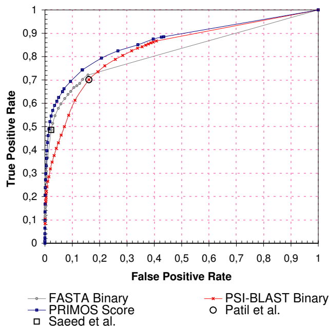
Figure 5 Comparison of Homology-Based Validation Schemes. Performance of the scoring scheme ('PRIMOS Score') in comparison to two conventional approaches (named 'FASTA Binary' and 'PSI-BLAST Binary' here), where a PPI is deemed as biologically relevant as soon as a single homologous PPI is found below a certain E-value. GSP PPIs comprised all PPIs from the Combined data set, the Random data set was used for the GSN PPIs. For the two binary schemes, we used FASTA and PSI-BLAST, respectively, to identify homologous PPIs and calculated the TPRs and FPRs as the fraction of GSP PPIs and GSN PPIs that had at least one homologous PPI below a sliding E-value threshold, ranging from 10^{-300} to 10 in this figure. Black rectangle: parameter settings from Saeed and Deane [23]. Black circle: parameter setting used by Patil and Nakamura [8]. The area under the curve (AUC) is 82%, 83%, and 86% for the FASTA, PSI-BLAST, and PRIMOS curve, respectively.
