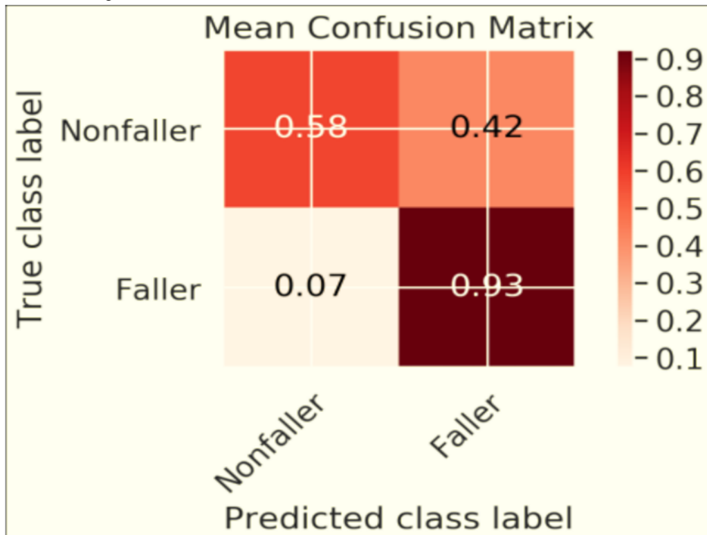
Figure 2. Confusion matrix averaged over all five models.
