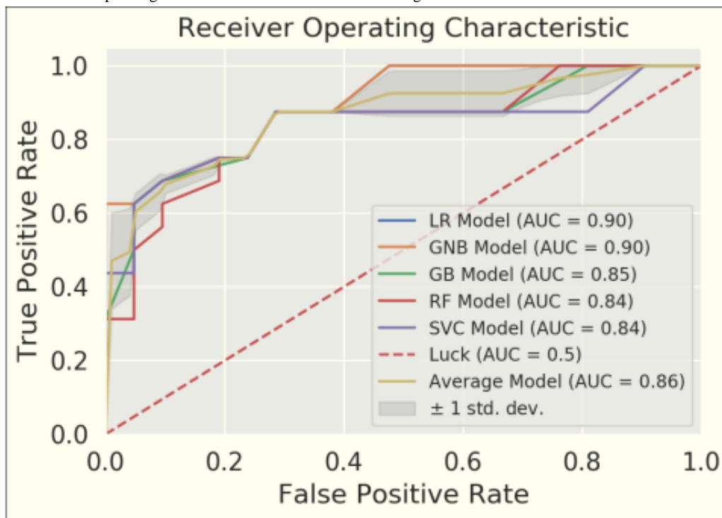
Figure 3. ROC curves and corresponding AUCs for the five models and the average over all five models.
