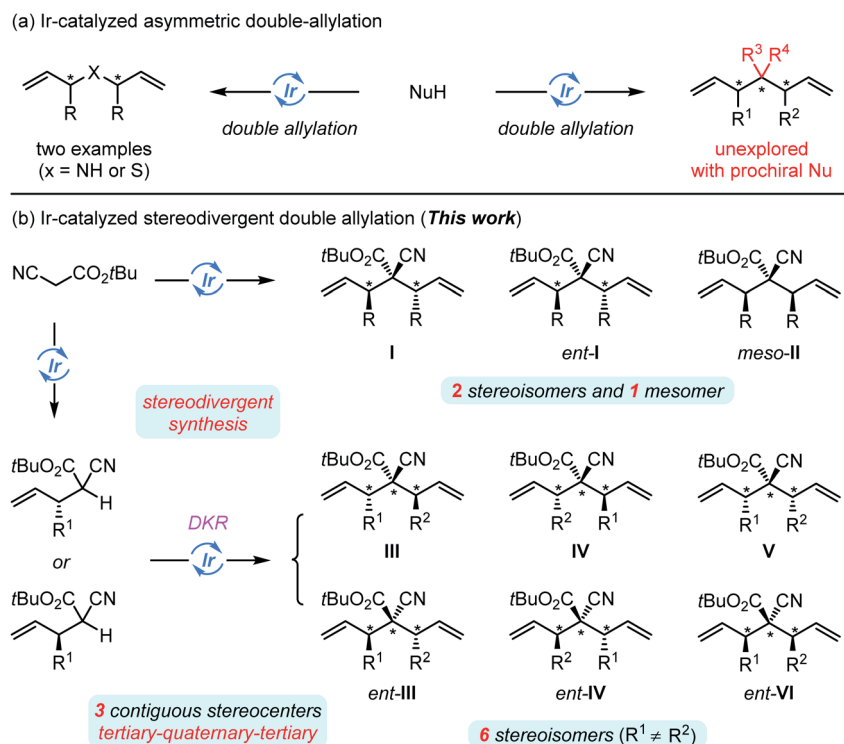
Scheme 2 Ir-catalyzed double-asymmetric allylic alkylation ((a) previous work) and stereodivergent double allylation ((b) this work).
