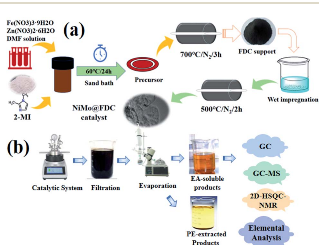
Fig. 1 (a) Illustration of NiMo@FDC catalyst preparation; (b) illustration of Kraft lignin catalytic depolymerization.
