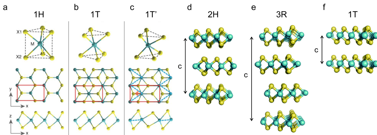
Fig. 1 Schematics of the polymorphs and stacking polytypes: (a–f) 1H, 1T, 1T', 2H, 3R, and 1T. Reproduced with permission from (a–c) ref. 60. Copyright 2014, Science; (d–f) ref. 62. Copyright 2015, Royal Society of Chemistry.
