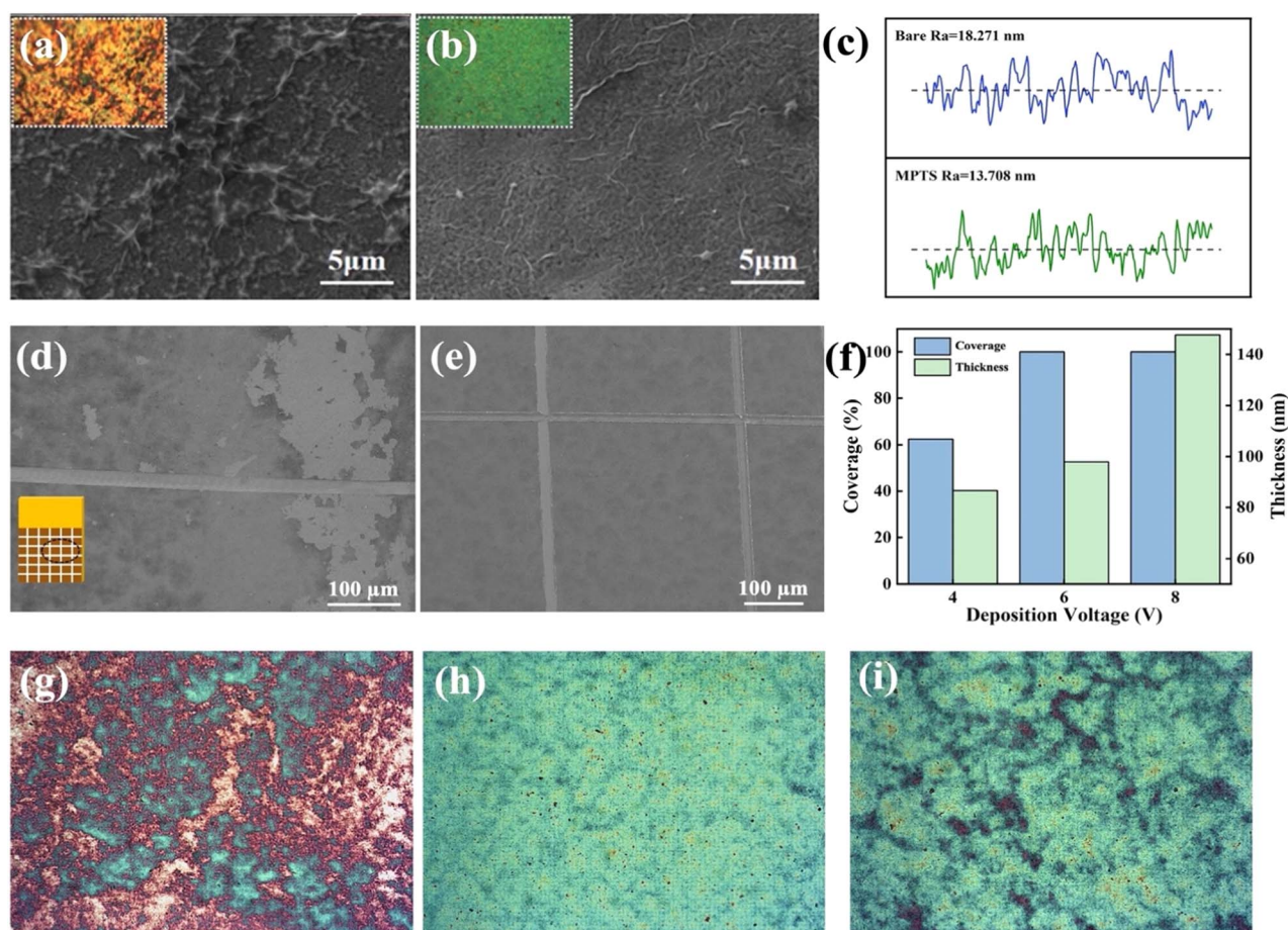
Fig. 3 SEM of GO film microstructure deposited on (a) bare copper surface and (b) MPTS-modified copper surface at 6 V for 5 min. (c) AFM line scan of roughness of deposited GO film with or without MPTS modification (three-dimensional AFM images are shown in ESI Fig. S3†). (d) GO-Cu surface and (e) GO-MPTS-Cu surface after adhesion tape test. (f) Histogram of variation of coverage and thickness with deposition voltage. The thickness was tested by a step profiler (DektakXT, Bruker) and the coverage is calculated roughly by the GO and bare copper area ratio in optical microscopies. The optical microscopy ( \times 1000 ) of GO film deposited at (g) 4 V, (h) 6 V, (i) 8 V.
