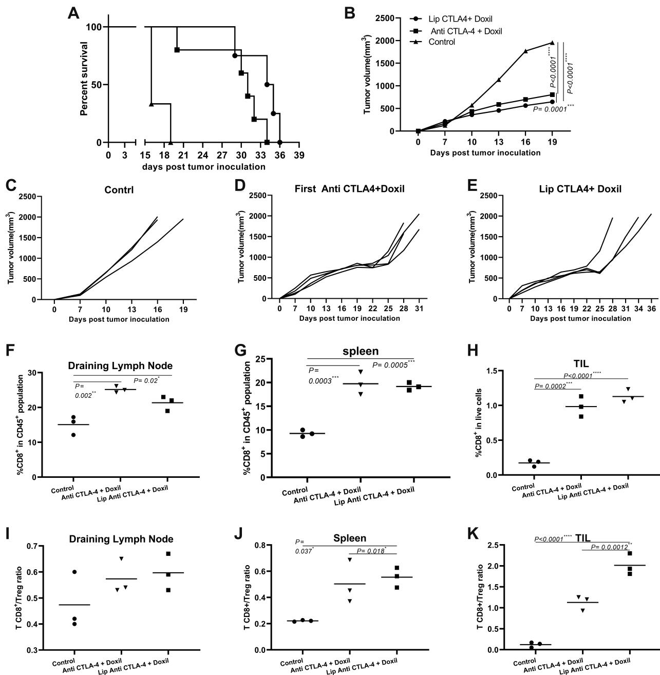
Figure 3 Liposomal delivery increases the efficiency of combination therapy of anti-CTLA-4 with Doxil. (A) survival analysis mice bearing B16 tumor, liposomal increases survival significantly in combination therapy when replaced with non-liposomal treatment, Mantel-Cox test shows statistically significant differences between treatment groups ( p < 0.001 ). (B) Comparison between tumor size of different groups, combining therapy with liposomal before Doxil reduced the tumor size in comparison to other groups. (C–E) Tumor size progression graph for each treatment groups, individually. (F) %CD8 + in CD 45 + population of DLN. (G) %CD8 + of in CD 45 + population spleen. (H) %CD8 + in live cells of tumor microenvironment. (I) TCD8 + /Treg ratio in DLN. (J) TCD8 + /Treg ratio in spleen. (K) TCD8 + /Treg ratio in TIL, liposomal administration before Doxil increased TCD8 + /Treg ratio compared to non-liposomal treatment (* p < 0.05 , ** p < 0.01 , *** p < 0.001 , **** p < 0.0001 ).
