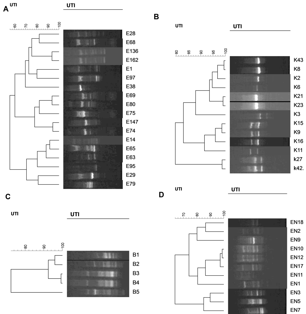
Figure 1 Genotyping of E. coli (A), K. pneumoniae (B), B. cepacia complex (C), and E. faecium strains (D) that met hospital-acquired infection criteria using RAPD-PCR.
