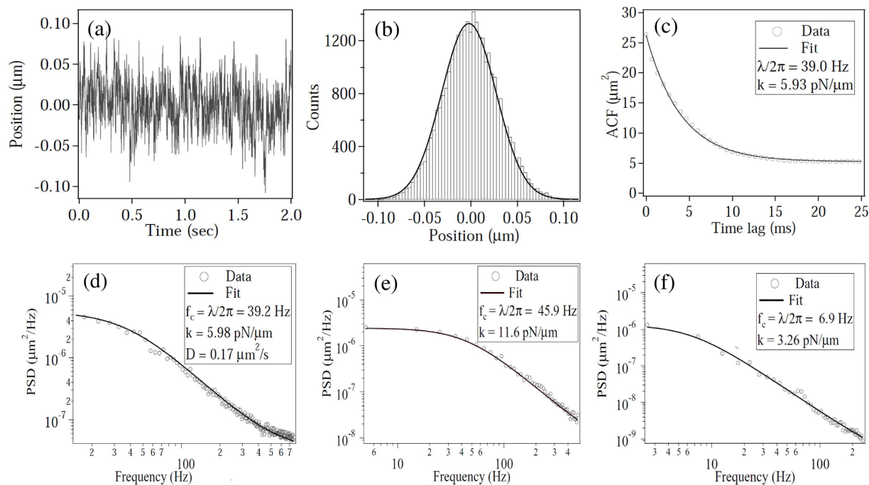
Figure 2. Discrete sample path and empirical statistics of an optically trapped Brownian polystyrene bead of radius a = 3 \mu\text{m} . Panel (a) shows discrete observations of one coordinate of the sample path, (b) the histogram of the position coordinate, (c) the autocorrelation function and (d) is the spectral density. Panel (e) and (f) are the spectral density for 5 and 10 \mu\text{m} diameter polystyrene spheres. The fits of \lambda from the both the autocorrelation and the spectral density depend, respectively, on the number of lags and the number of frequencies used. The guidelines in ref. 7 and 18 are followed in obtaining the fits.
