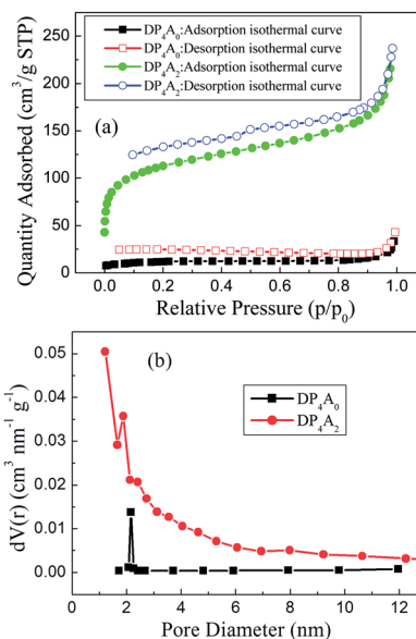
Fig. 3 (a) Nitrogen adsorption–desorption isotherms measured at 77 K for DP 4 A 0 and DP 4 A 2 ; (b) the BJH pore size distribution profiles of DP 4 A 0 and DP 4 A 2 calculated using the NLDFT method.
