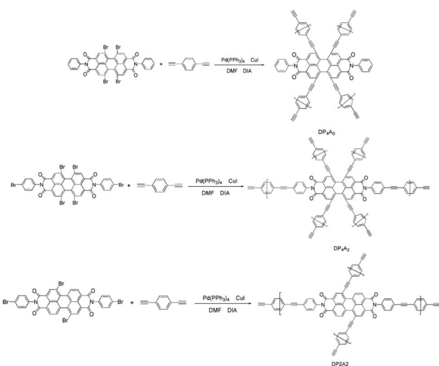
Scheme 1 Synthesis of DP 4 A 0 , DP 4 A 2 , and DP 2 A 2 via Sonogashira–Hagihara cross-coupling reactions.
