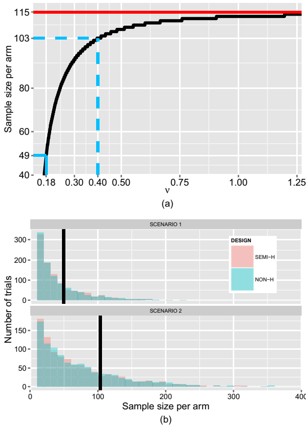
Figure 1 (a) Sample size per arm (SS) vs. difference in improvement of topiramate (TPM) over placebo between children ( \delta_P ) and adults ( \delta_A ) expressed in terms of SD of the prior distribution on \delta_P and \delta_A ( v ). The red line represents the sample size per arm of a classical parallel frequentist design, azure lines indicate the value of v and the corresponding SS of the Bayesian design (BD) in scenario 1 (solid line) and 2 (dotted line). (b) Histograms of SSs obtained at each of the 1,000 clinical trial simulation of the Bayesian sequential design in the non-hierarchical (NON-H; green histogram) and semi-hierarchical (SEMI-H; pink histogram) framework for scenario 1 (upper panel) and 2 (lower panel). The black vertical lines indicate SS of the BD in the two scenarios.
