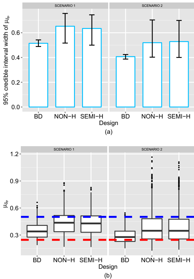
Figure 3 (a) Bar chart plot of the median 95% credible interval width of treatment difference estimates ( \mu_{\delta_p} ) obtained at each of the 1,000 clinical trial simulation of the Bayesian design (BD), the Bayesian sequential design with a non-hierarchical (NON-H) and a semi-hierarchical (SEMI-H) framework for scenario 1 (left panel) and 2 (right panel). The upper and lower “hinges” correspond to the first and third quartiles of 95% confidence intervals widths. (b) Boxplots of \mu_{\delta_p} obtained at each simulation of the BD, the NON-H and the SEMI-H for scenario 1 (left panel) and 2 (right panel). The blue and red dotted lines represent the adult and pediatric treatment effects difference between topiramate and placebo (obtained from the pharmacokinetic-pharmacodynamic model), respectively.
