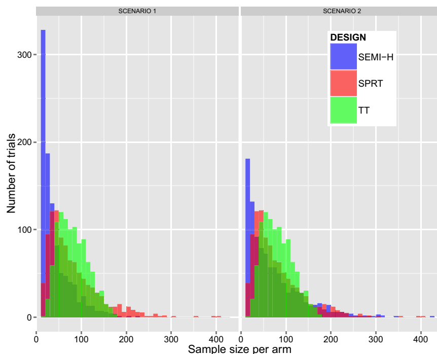
Figure 4 Histograms of the sample sizes per arm obtained at each of the 1,000 clinical trial simulation of the semi-hierarchical (SEMI-H) Bayesian sequential design (blue histogram), sequential probability ratio test (SPRT; red histogram), and the triangular test (TT; green histogram).
