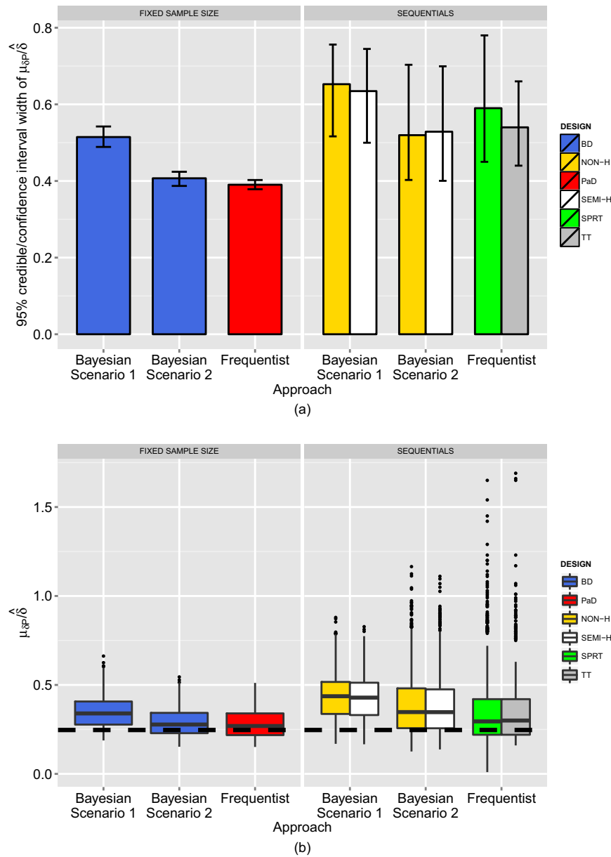
Figure 5 Bar chart plot of the 95% credible (Bayesian) and confidence (frequentist) interval width of treatment difference estimates in pediatrics ( \mu_{\delta_p} for Bayesian designs (BDs) and \hat{\delta} for frequentist ones) (a) and boxplot of \mu_{\delta_p} and \hat{\delta} (b) obtained at each of the 1,000 clinical trial simulation of the BD (blue bar), parallel design (PaD; red bar), Bayesian sequential design with a non-hierarchical (NON-H; yellow bar), and a semi-hierarchical (SEMI-H; white bar) framework, sequential probability ratio test (SPRT; green bar), and triangular test (TT; gray bar). The upper and lower “hinges” in subfigure (a) correspond to the first and third quartiles of 95% credible/confidence intervals widths. The dashed horizontal black line represents the pediatric treatment effect difference between topiramate and placebo obtained from the pharmacokinetic-pharmacodynamic (PK-PD) model (0.2467).
