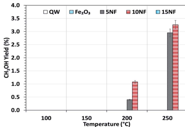
Fig. 6 \text{CH}_3\text{OH} yield as a function of the reaction temperature. Reaction conditions: catalyst, 0.5 g; \text{H}_2/\text{CO}_2 = 75/25 , flow rate, 100 mL min; P = 1 atm.
