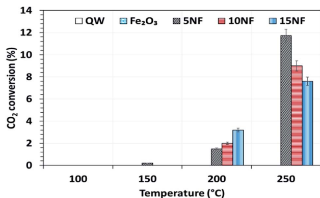
Fig. 5 The influence of temperature on \text{CO}_2 conversion for the different catalysts. Reaction conditions: catalyst, 0.5 g; \text{H}_2/\text{CO}_2 = 75/25 , 100, 25, 100 mL min; P = 1 atm.
