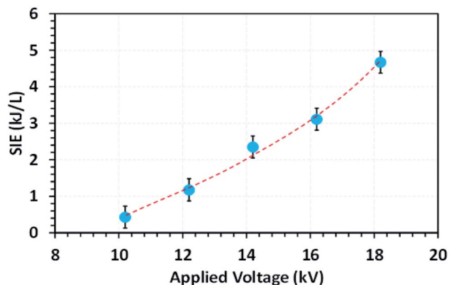
Fig. 4 The evolution of the SIE as a function of the applied voltage (feed flow rate: 100 \text{ mL min}^{-1} , \text{CO}_2/\text{H}_2 = 1 : 3 , frequency: 50 Hz).
