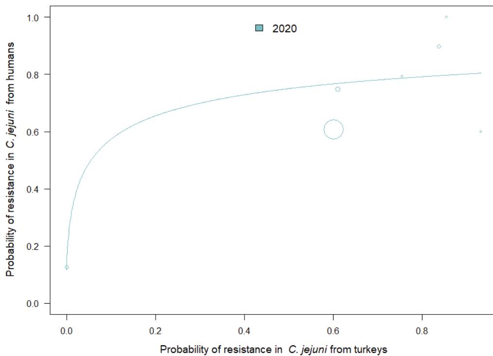
FIGURE 33 Probability of resistance to fluoroquinolones in Campylobacter jejuni from humans and turkeys, EU/EEA, 2020 (see Table 27). The figure displays results of logistic regression analyses. Bubbles represent the countries included in the analysis. The size of the bubbles indicates the amount of available resistance data per country.
