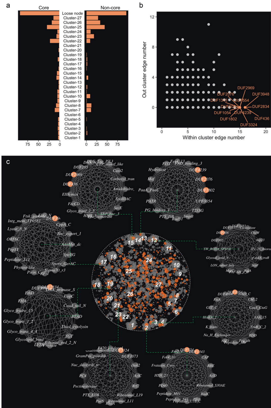
Fig. 6 Predicting functions of genes encoding domain of unknown functions ( DUF ). a The distribution of DUF genes. b Identifying the
