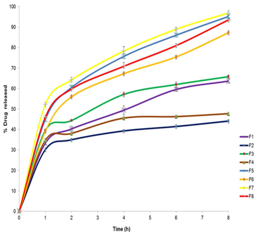
Figure 7 The in vitro release profile of AKBA-loaded SNVs, ( n = 3 ). Abbreviations: AKBA, 3-acetyl-11-keto- \beta -boswellic acid; SNVs, spanlastic nanovesicles.
