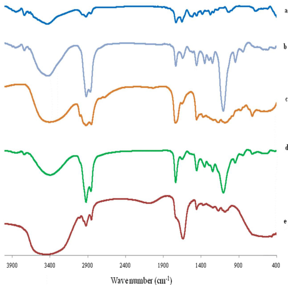
Figure 11 FTIR spectrum of (A) AKBA, (B) Tween 80, (C) Span 60, (D) Plain spanlastic and (E) the optimized AKBA-loaded SNVs. Abbreviations: AKBA, 3-acetyl-11-keto- \beta -boswellic acid; SNVs, spanlastic nanovesicles.
