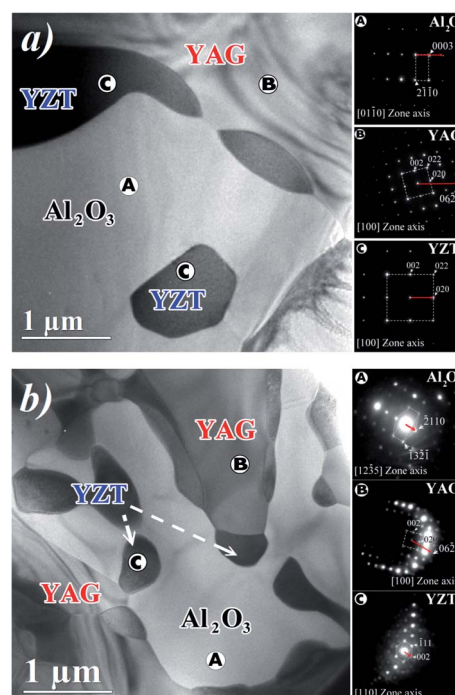
Fig. 7 Transversal TEM micrograph of \text{Al}_2\text{O}_3\text{-YAG-ZrO}_2 eutectic microstructure: (a) 0.1 and (b) 1 \text{ mm min}^{-1} . The black region is the \text{ZrO}_2 phase, the light grey region is the YAG phase and the dark grey is the \alpha\text{-Al}_2\text{O}_3 phase. (A), (B) and (C) regions correspond to the position of SAED measurement.
