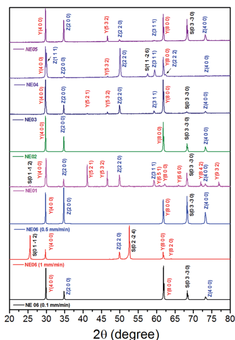
Fig. 6 Room-temperature bulk XRD patterns of the transversal sections of \text{Al}_2\text{O}_3/\text{YAG}/\text{ZrO}_2 eutectic and off eutectic composition. The off eutectic samples were grown under a pulling rate 0.5 \text{ mm min}^{-1} and three pulling rates ( 0.1 , 0.5 and 1 \text{ mm min}^{-1} ) were used for the eutectic composition.
