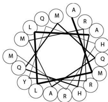
Figure 3. Helical wheel representation of Polystira albida turrtoxins (PaIAa) residues 33–50, which form one of two predicted \alpha -helices.
