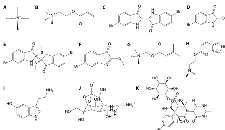
Figure 4. Small molecule compounds discussed in this review. (A) Tetramine, (B) acrylylcholine, (C) Tyrian purple, (D) 6-bromoisatin, (E) tyriverdin, (F) tyrindoleninone, (G) senecioclholine, (H) urocanycholine (murexine), (I) serotonin (J) tetrodotoxin, and (K) surugatoxin.
