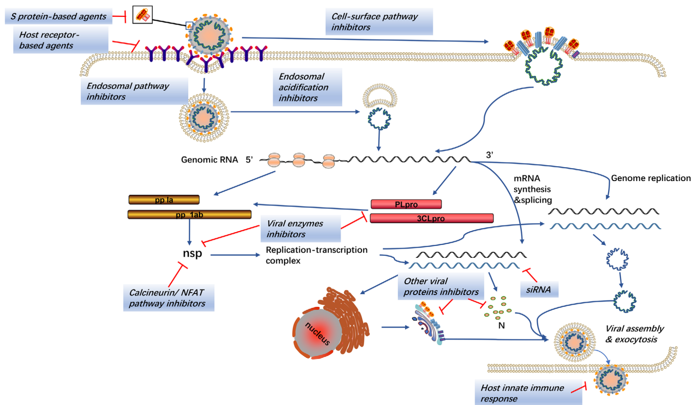
FIGURE 3 Mechanisms of current anti-CoV therapeutic agents
