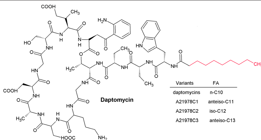
Figure 1 The chemical structure of daptomycin and other A21978C factors.
