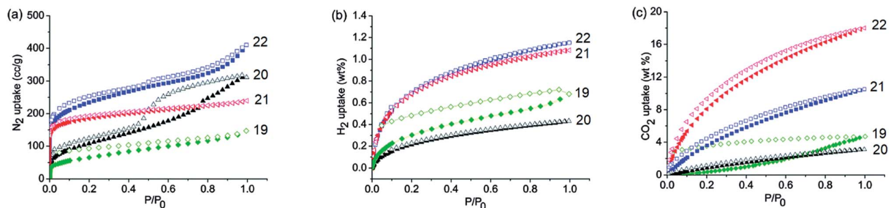
Fig. 10 Gas adsorption isotherms of 19–22. (a) \text{N}_2 adsorption isotherms at 77 K, (b) \text{H}_2 adsorption isotherms at 77 K and (c) \text{CO}_2 adsorption isotherms at 273 K and 1 bar. Reproduced from ref. 31 with permission. Copyright© 2015, Royal Society of Chemistry.
