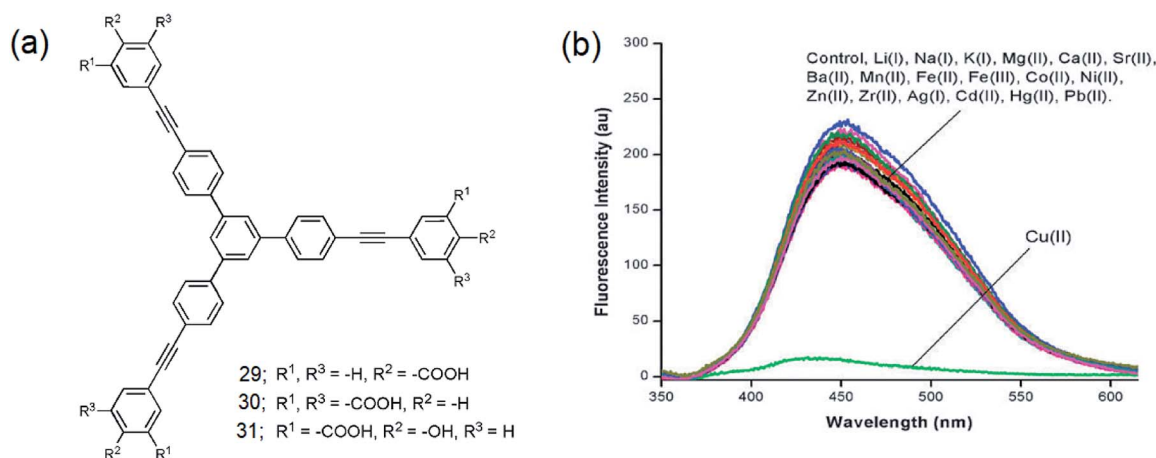
Fig. 17 (a) Structures of 29–31 and (b) photoluminescence spectra of 31 (1.0 × 10 -3 M) in the presence of various metal ions (10.0 × 10 -5 M). Cu(II) selectively quenches the photoluminescence. Reproduced from ref. 24 with permission. Copyright© 2011, Royal Society of Chemistry.
