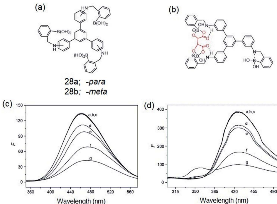
Fig. 16 (a) C 3 -symmetric tris-boronic acids, (b) proposed complex of α-hydroxycarboxylic acid with the sensor molecule, (c) PL spectra of 28a (1.4 × 10 -2 mM, λ ex = 297 nm) and (d) 28b (6 × 10 -2 mM, λ ex = 257 nm) in the presence of 5.0 mM of different analytes (a) free, (b) D-glucose, (c) D-galactose, (d) galacturonic acid, (e) lactic acid, (f) malic acid, (g) tartaric acid. Reproduced from ref. 68 with permission. Copyright© 2008, Elsevier Ltd.
