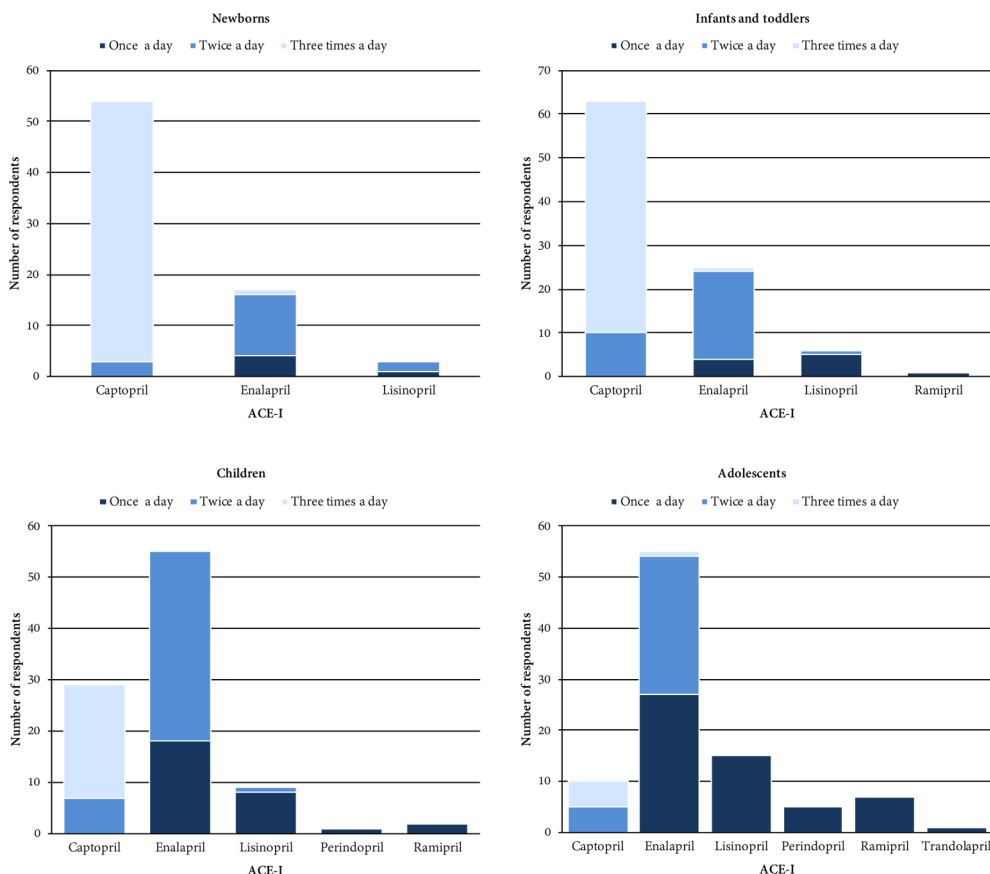
Figure 5 Dosing frequency of ACE-I maintenance dose reported for ACE-I of choice selected for each age group. Age groups were defined as follows: newborns 0–27 days, infants and toddlers 28 days to 23 months, children 2–11 years and adolescents 12–18 years. 42 Captopril appeared to be most commonly prescribed three times per day and enalapril two times a day in all paediatric age groups except for adolescents. In this age group, the prevalence of prescribing enalapril once a day was similar to two times a day prescribing. Similarly, the percentage of clinicians reporting captopril administration two times and three times a day for adolescents was as high. Participants who reported using lisinopril, perindopril, ramipril and/or trandolapril prescribe these ACE-Is in single daily doses in virtually all cases. Answer option ‘4 times per day’ was also provided, but this was not selected in any case. One of the 30 participants that reported using captopril for children did not specify any dosing frequency. ACE-I, angiotensin-converting enzyme inhibitor.
