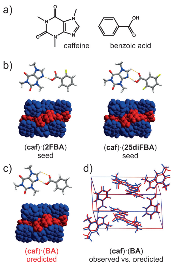
Figure 10. a) Molecular structure of caffeine ( caf ) and benzoic acid ( BA ). b) Cocrystals as heteronuclear seeds: cocrystals composed of caffeine ( caf ), 2-fluorobenzoic acid ( 2FBA ), and 2,5-difluorobenzoic acid ( 25diFBA ). c) Predicted lowest-energy crystal structure of ( caf )·( BA ). d) Overlay of the isomorphous lowest-energy predicted and obtained ( caf )·( BA ) cocrystal (red: predicted, blue: observed).
