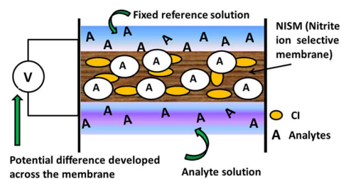
Fig. 14 Sensing mechanism for the membrane.
