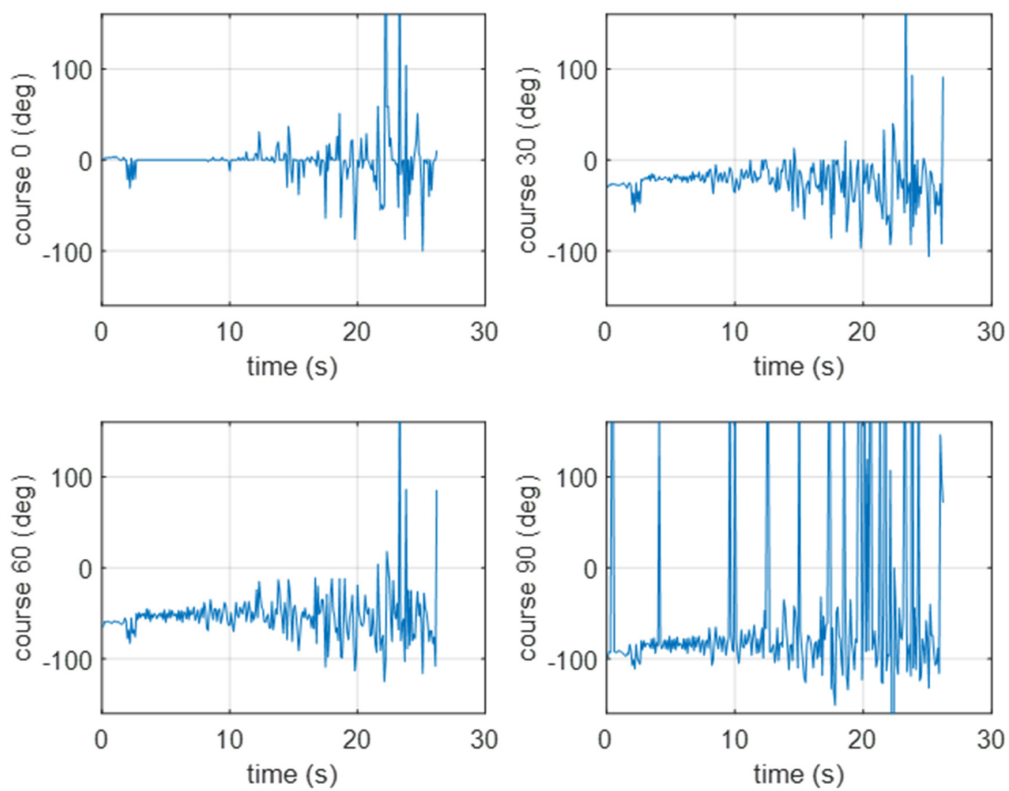
Figure 11. Results of the bearing estimation using the cross-correlation method (for a pontoon moving away from the BUUV2 at 0, 30, 60, or 90 [deg]).
