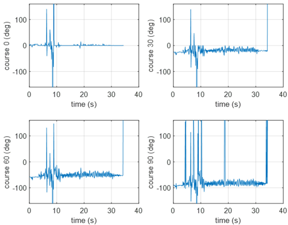
Figure 10. Results of the bearing estimation using the cross-correlation method (for a pontoon approaching the BUUV2 at 0, 30, 60, or 90 [deg]).
