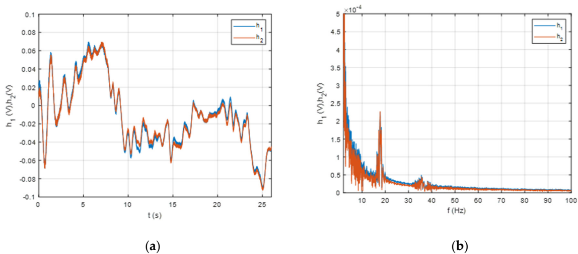
Figure 2. Measured signals from the two hydrophones ( h_1 and h_2 ): (a) the time domain; (b) the frequency domain.
