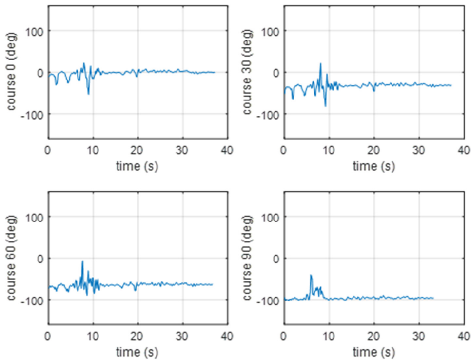
Figure 12. Results of the bearing estimation using the cross-zero method (for a pontoon approaching the BUUV2 at 0, 30, 60, or 90 [deg]).
