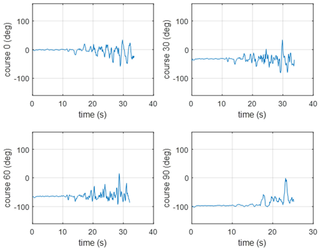
Figure 13. Results of the bearing estimation using the cross-zero method (for a pontoon moving away from the BUUV2 at 0, 30, 60, or 90 [deg]).
