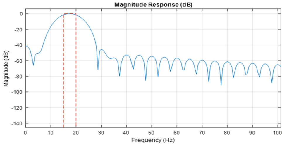
Figure 7. The passband linear phase filter.
