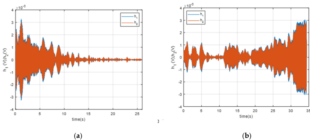
Figure 8. The signals measured after filtration with the passband linear phase filter in terms of the source of the sound: (a) approaching the BUV; (b) departing the BUV.
